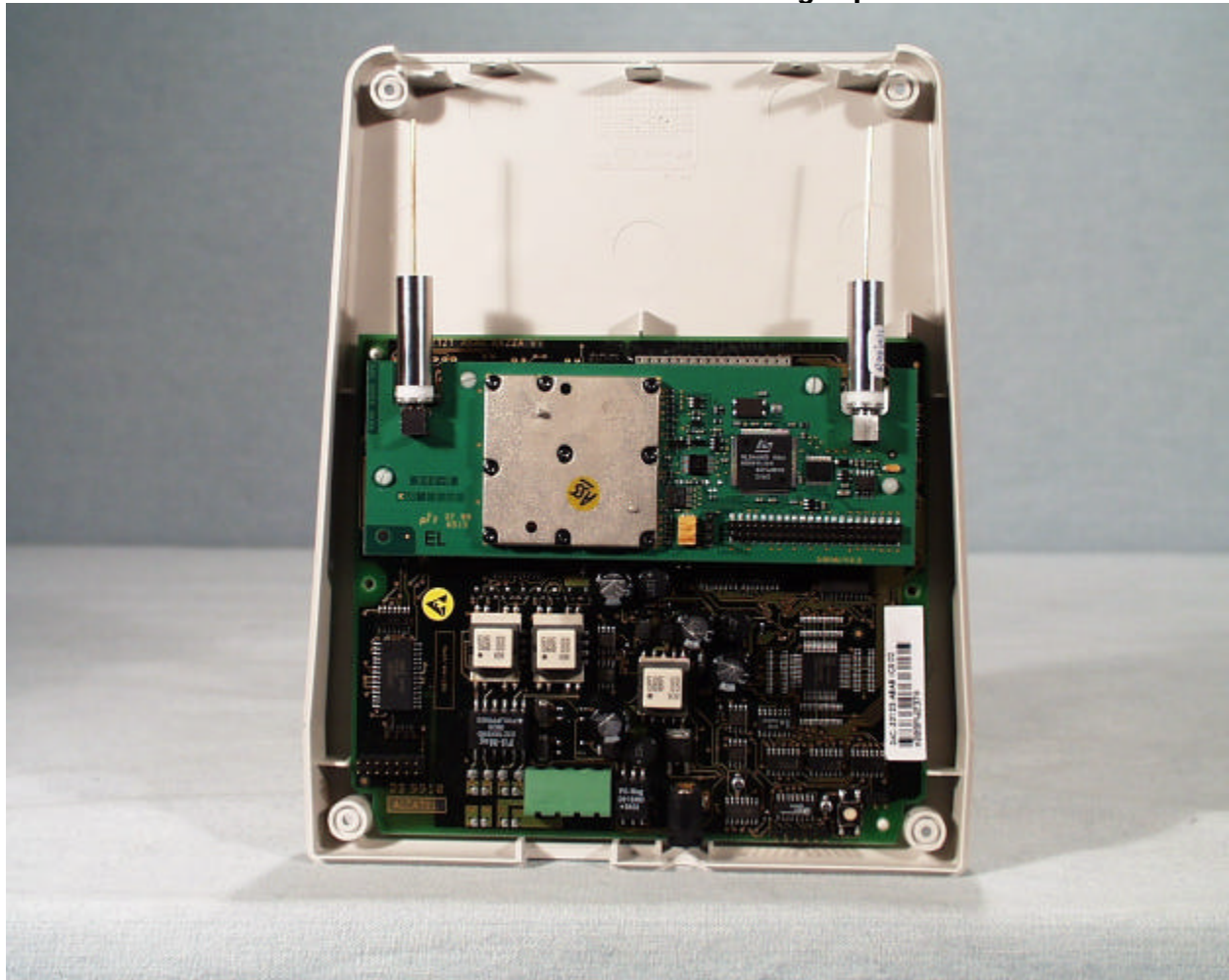
Inside View of the IBS / 4070 IO-3AC36116
