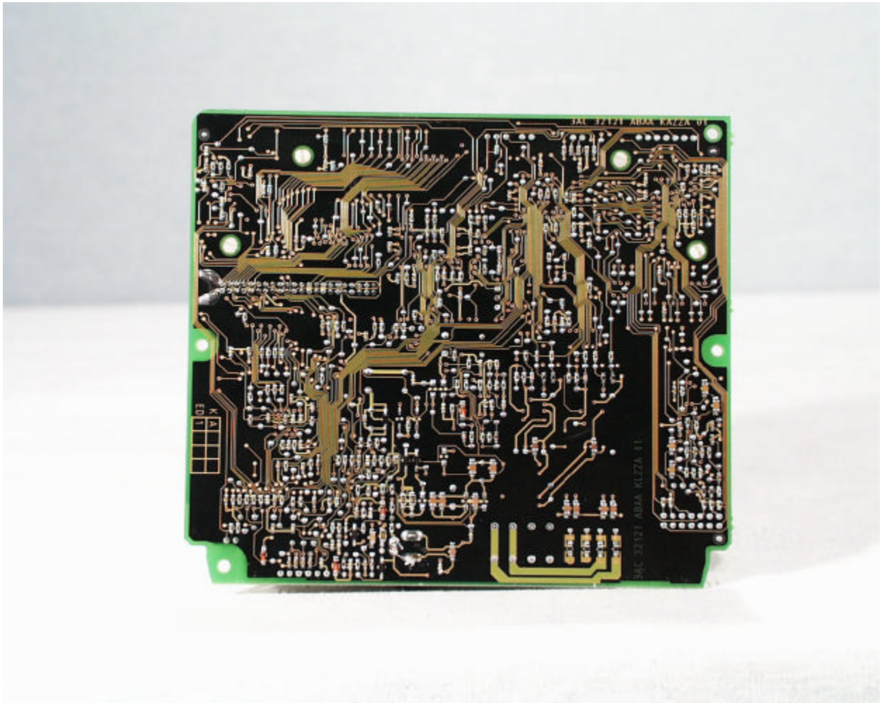
Back view of the radio board
