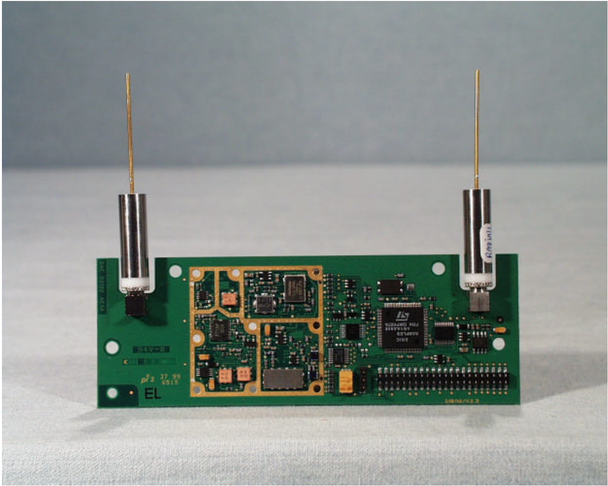
Front view of the antenna board (without RF cans)
