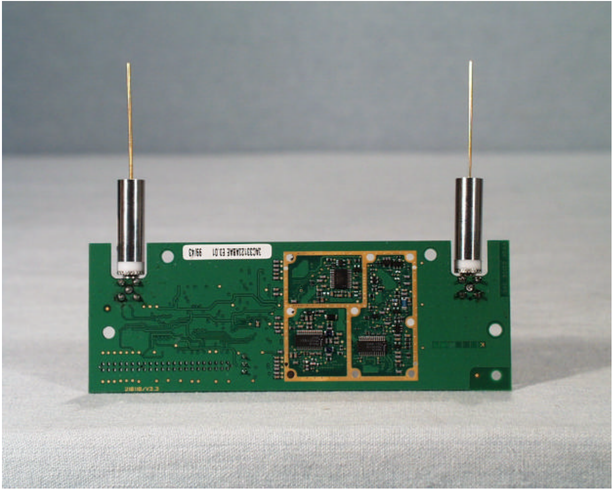
Back view of the antenna board (without RF cans)
