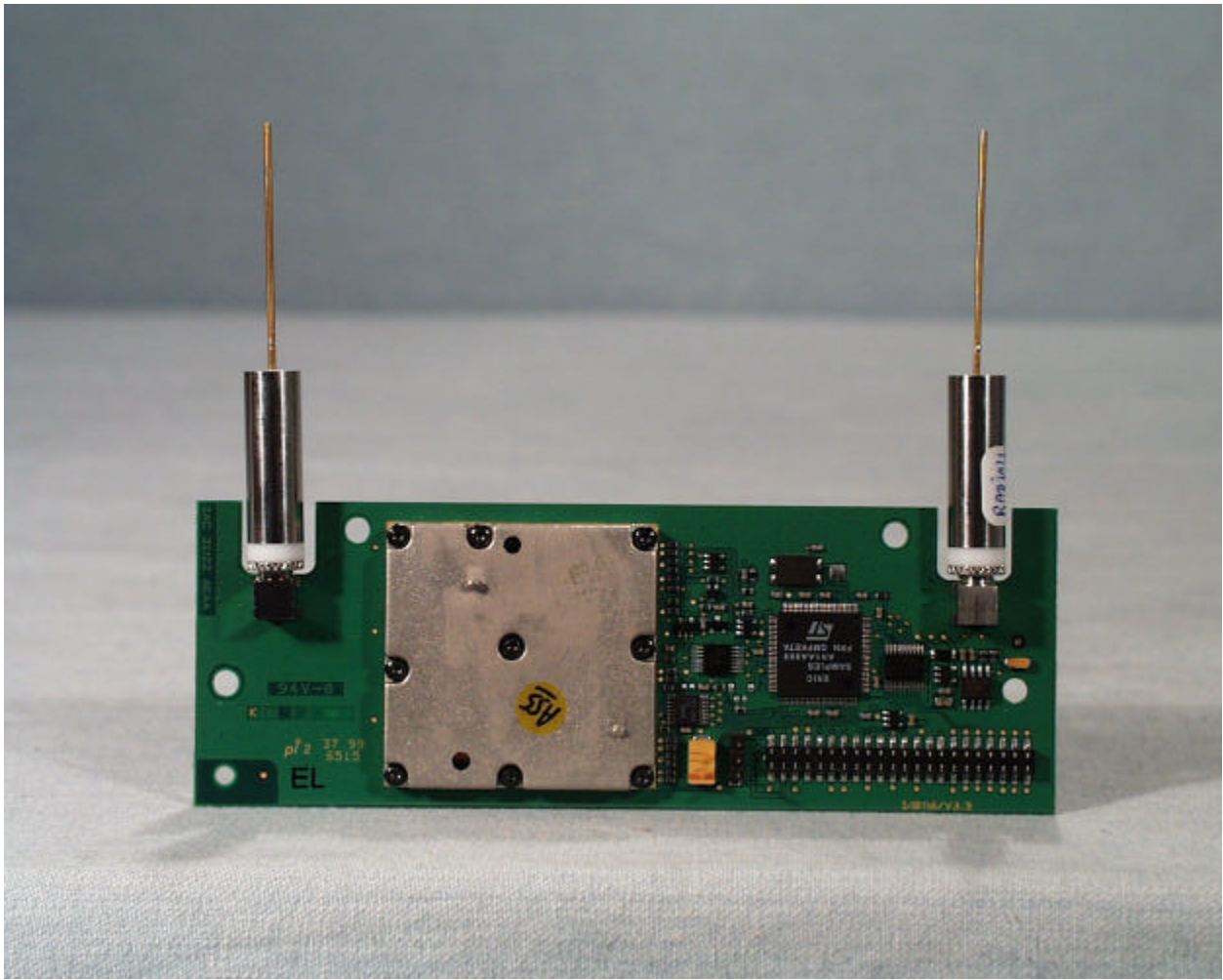
Front view of the antenna board (with RF cans)
