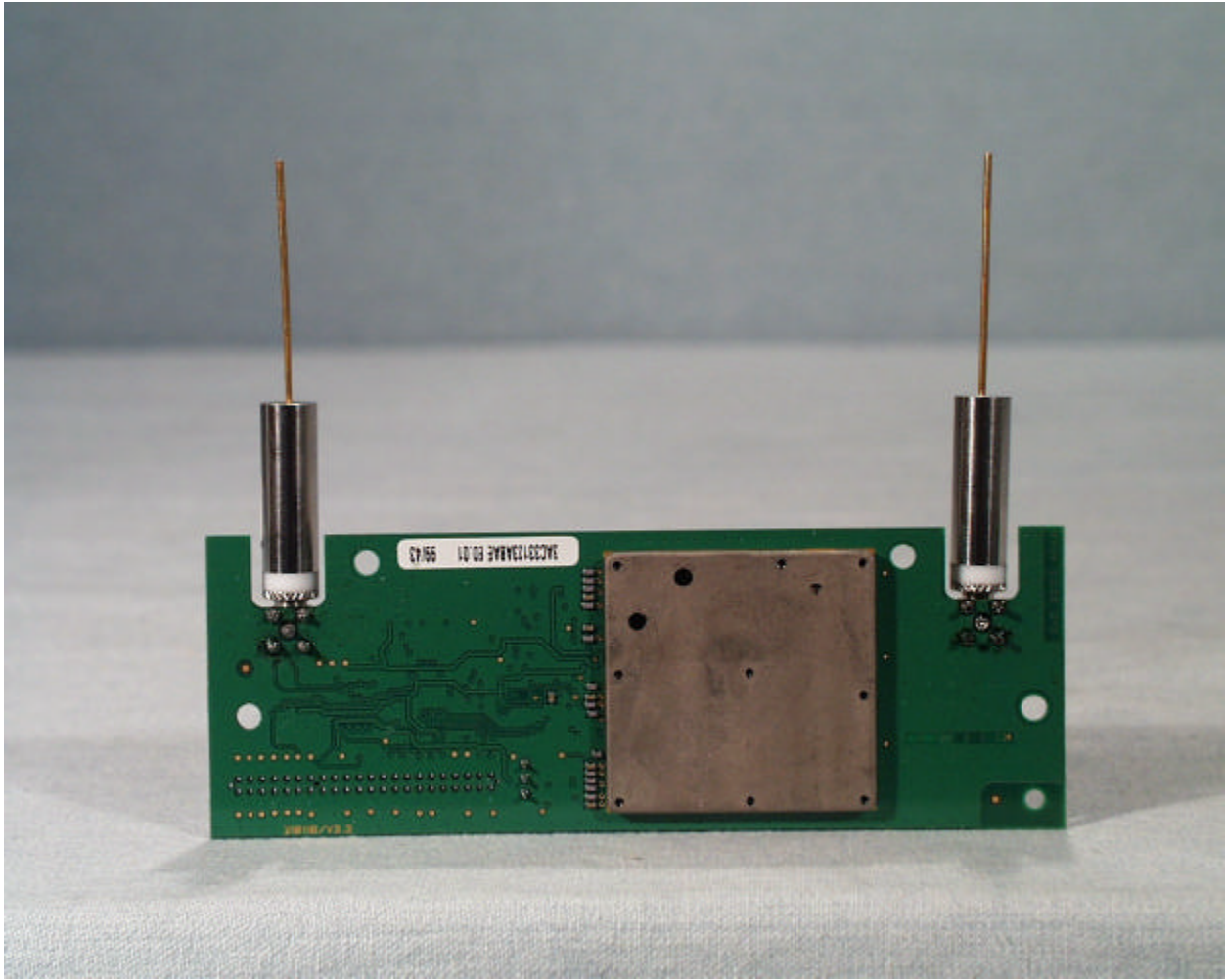
Back view of the antenna board (with RF cans)
