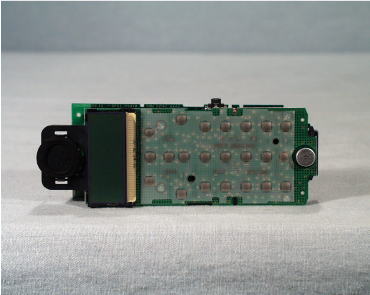
Front view of the keypad board
