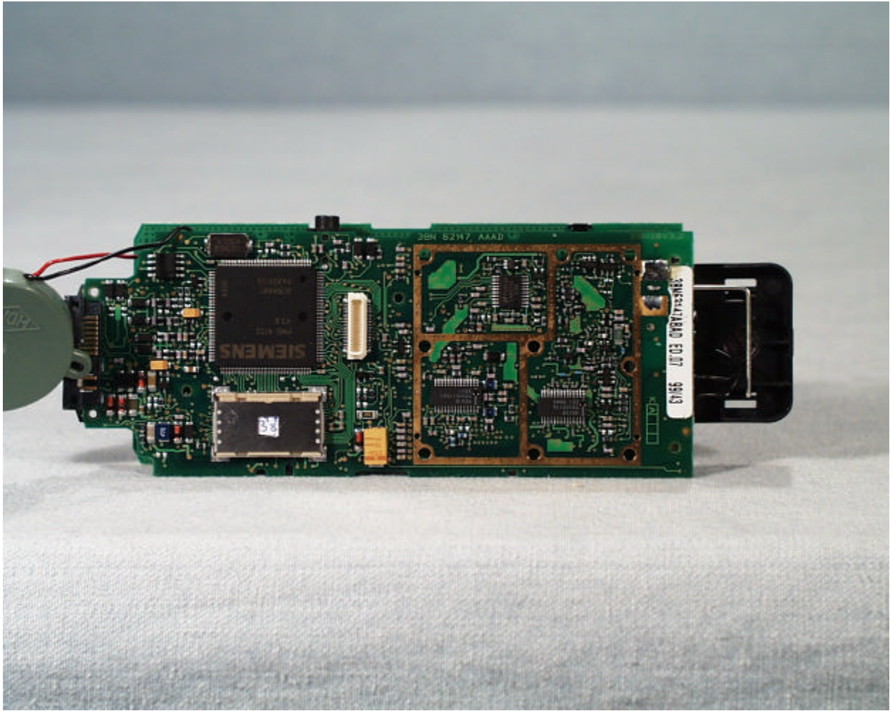
Back view of the radio board (without RF cans)
