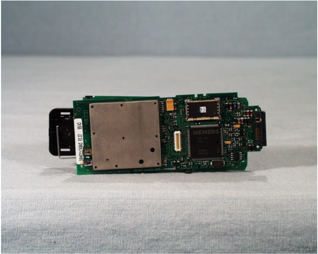
Back view of the radio board (with RF cans)
