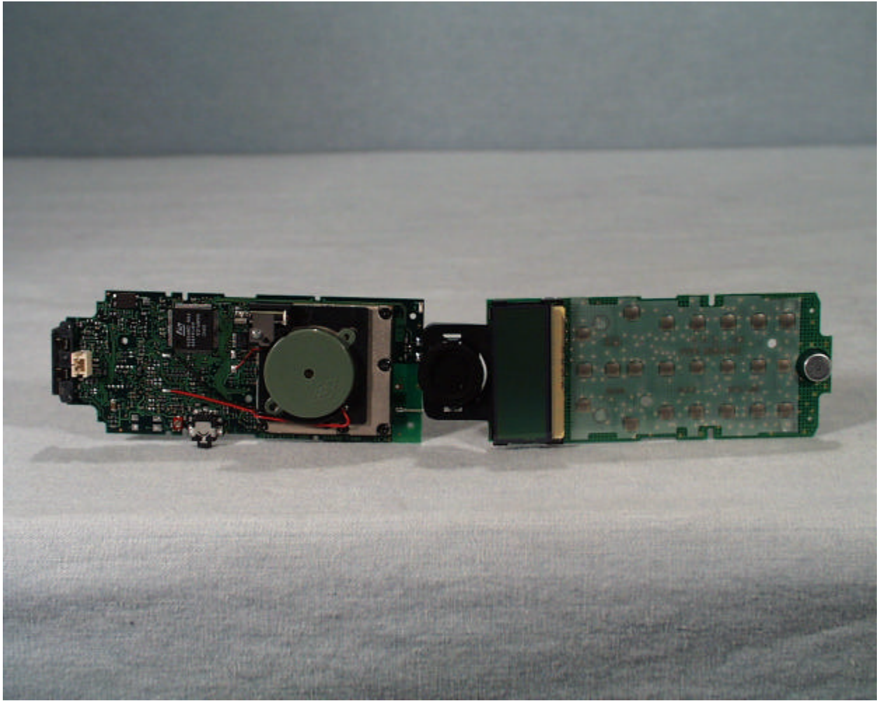
Front view of the radio board and keypad board
