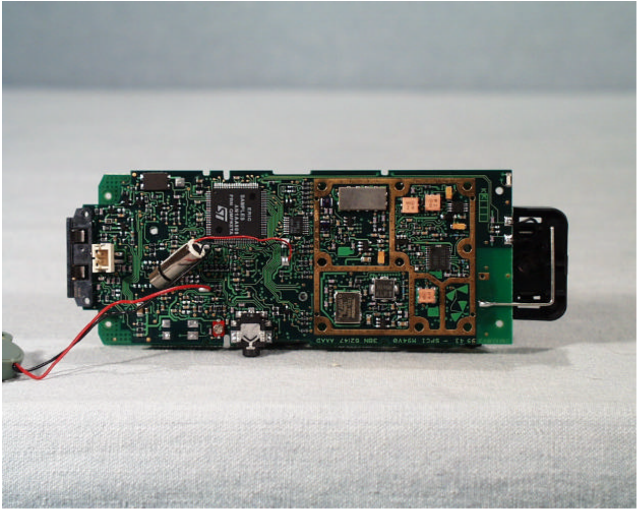
Front view of the radio board (without RF cans)
