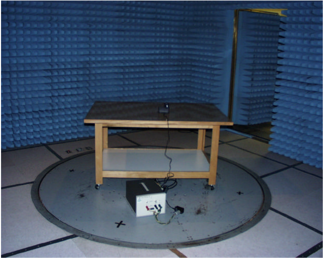
Back View of Worst Case Radiated and Line Conducted Emissions Test Set-up
