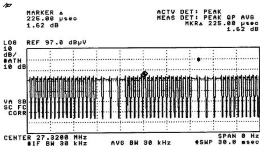
Figure C [Short Pulse]
