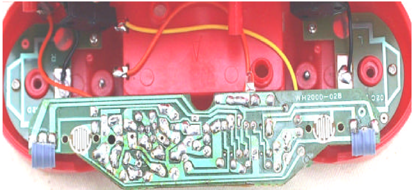
FCC ID: OYY98188 BOTTOM VIEW OF THE PRINTED WIRING BOARD
