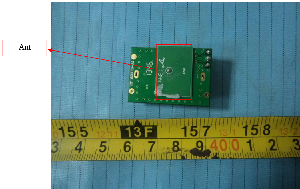
EUT – Main Bottom View
