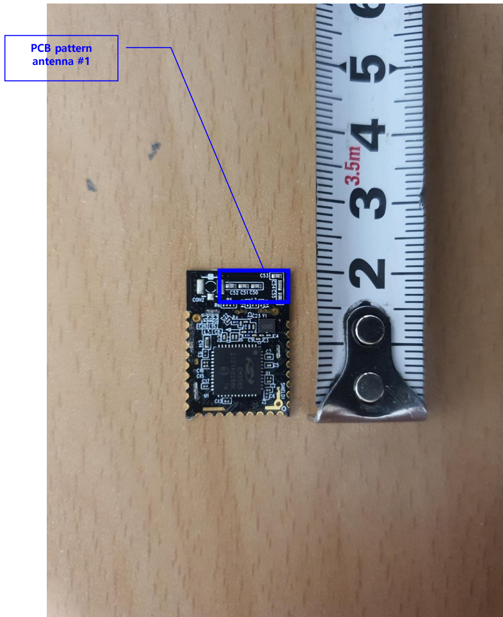
< Main board Top view #1 >
