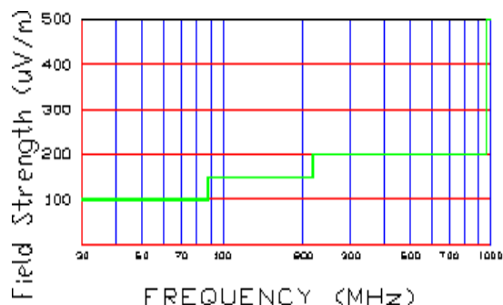
Figure 9. Spurious Radiated Limits at 3 meters
