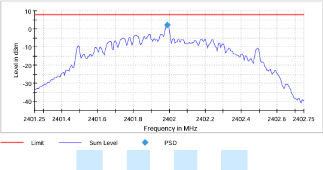
Power Density Plot on configuration : Lowest channel (2 402 MHz)
