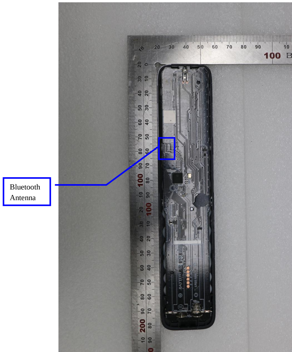
< Inside view #1 >
