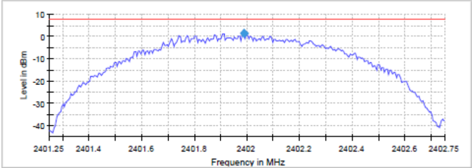
Power Density Plot on configuration : Lowest channel (2 402 MHz)
