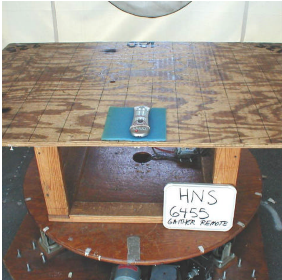
Figure 4: Radiated Emission Test Configuration, X-Axis
