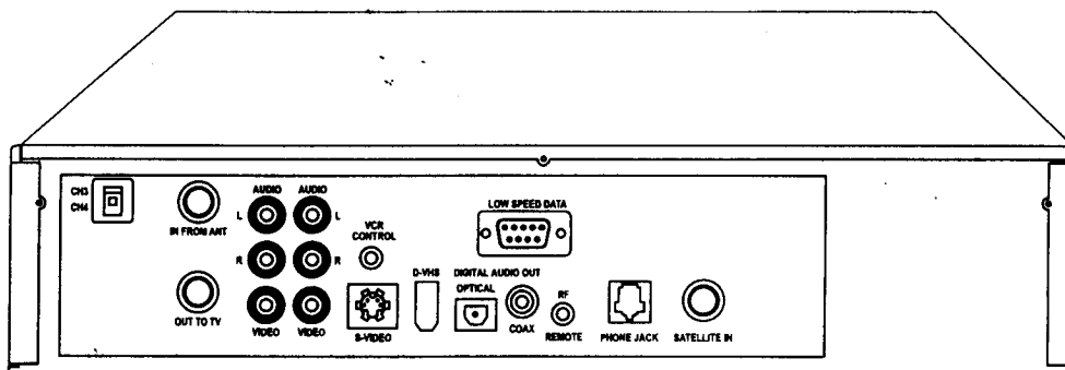
The rear of the digital satellite receiver.
