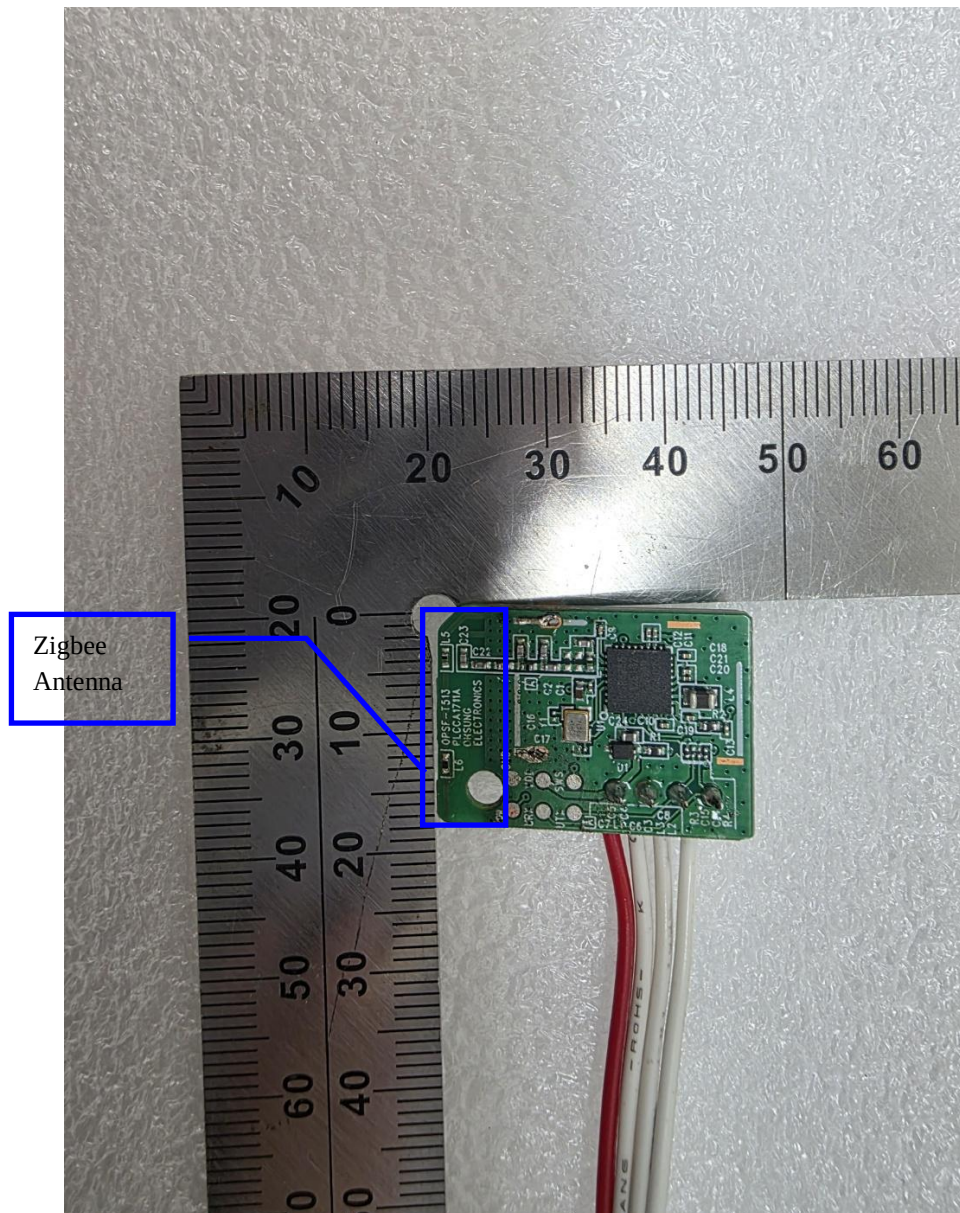
< Main board Top view >
