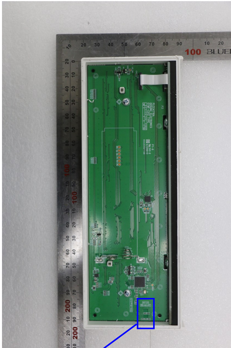
Bluetooth Antenna
