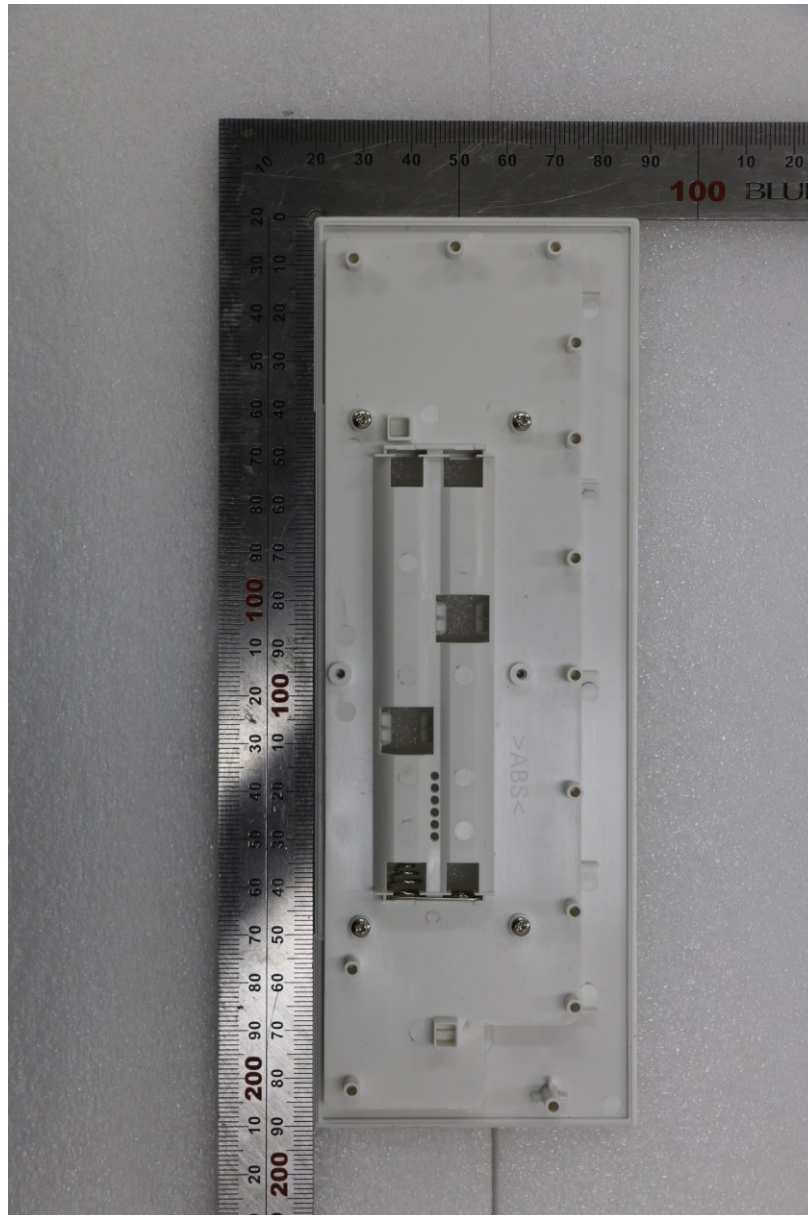
< Inside view #3>
