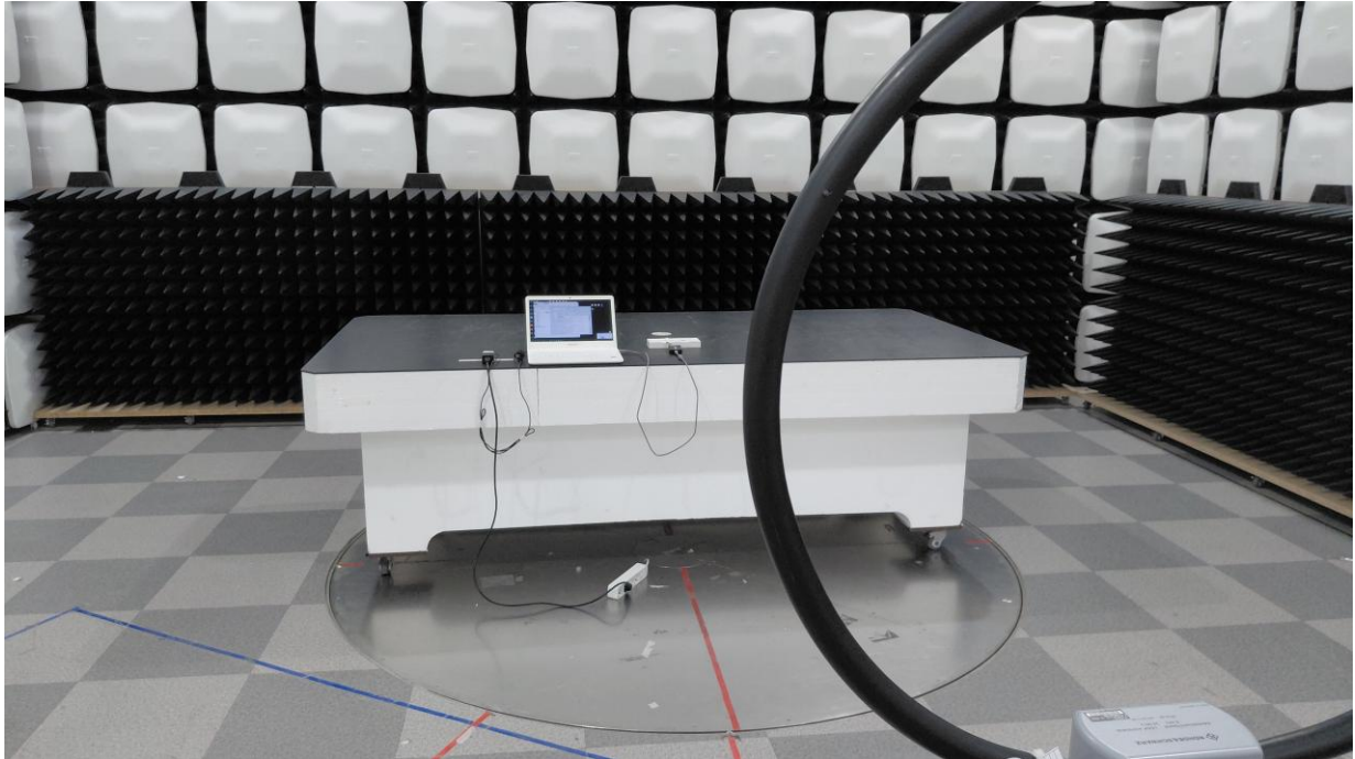
■ Radiated Test Picture: Below 30 MHz
