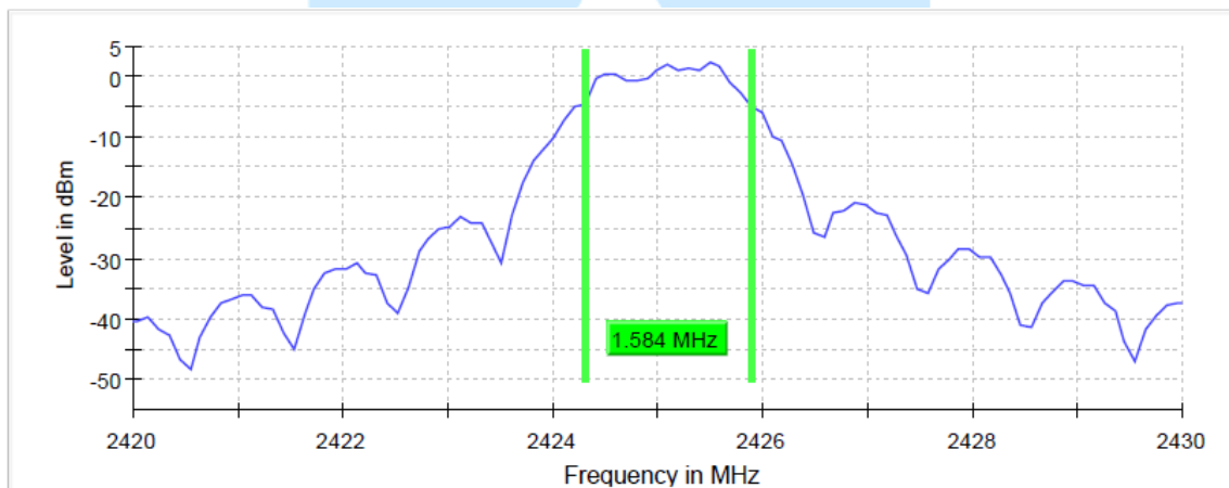
6 dB Bandwidth Plot on Configuration : Lowest channel (2 425 MHz)
