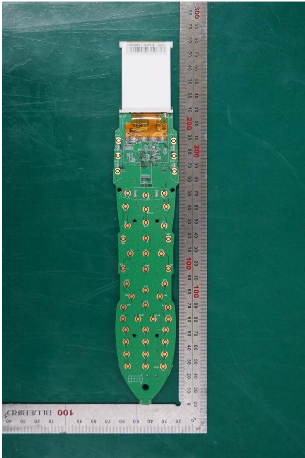
< Main board bottom view remove key sticker >
