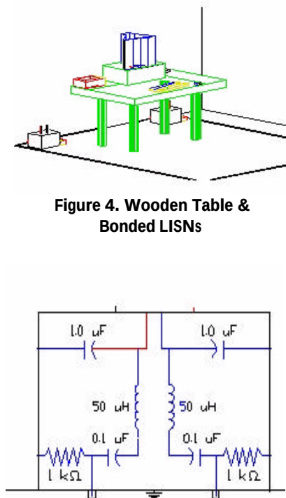
Figure 5. LISN Schematic Diagram
