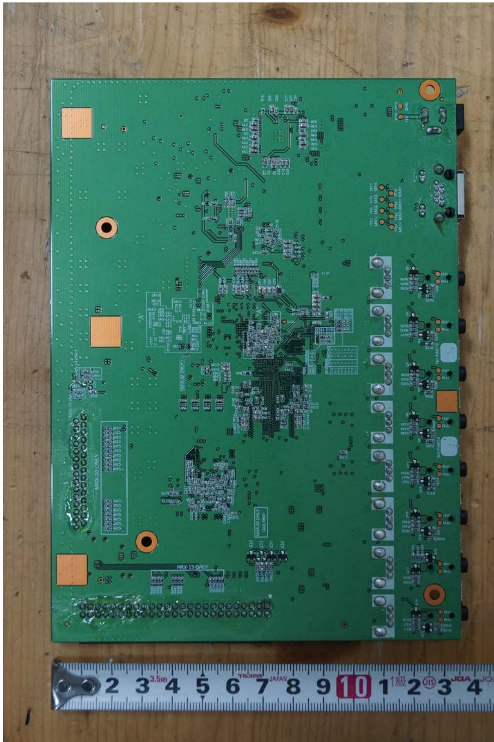
< Bottom of Main board >
