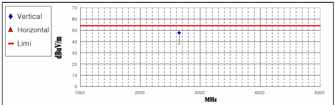
&lt; Fig 6. Radiated Emission result (1000MHz ~ 5000MHz)&gt;
