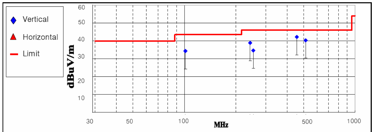
< Fig 7. Radiated emission result >
