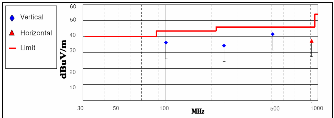
&lt; Fig 5. Radiated emission result (30MHz ~ 1000MHz)&gt;
