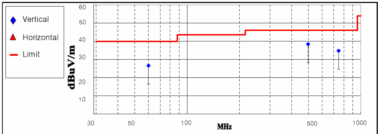
< Fig 8. Radiated emission result >
