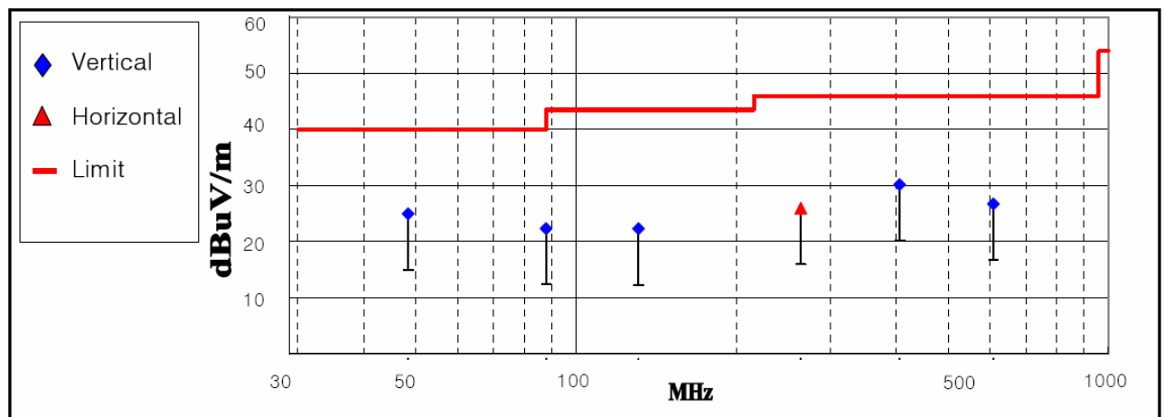
&lt; Fig 5. Radiated emission result (30MHz ~ 1000MHz)&gt;
