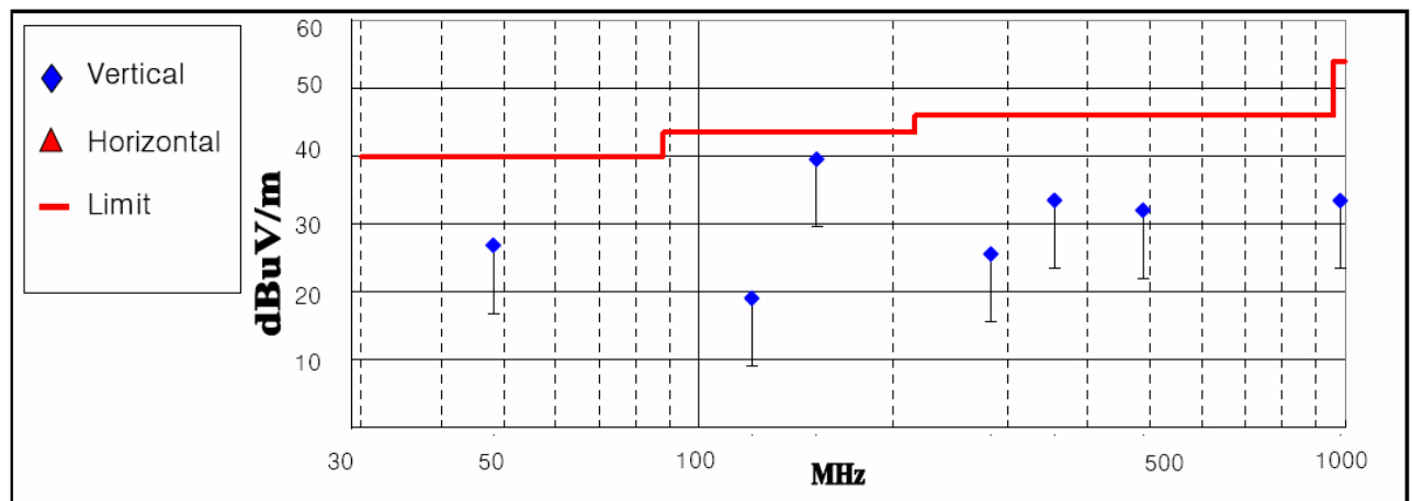
< Fig 7. Radiated emission result >
