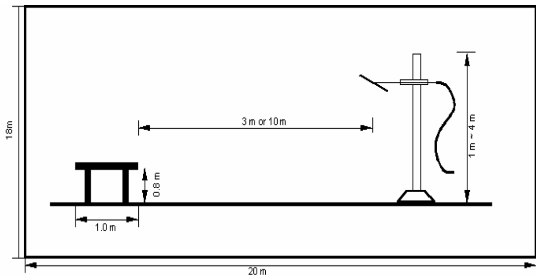
Fig 3. Dimensions of Open Site Test Area
