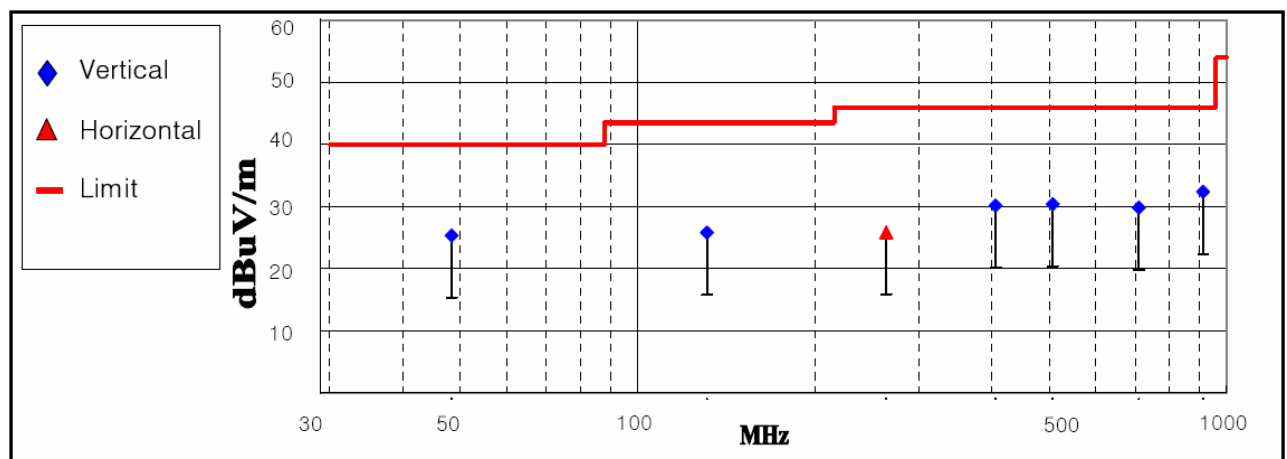
< Fig 6. Radiated emission result >
