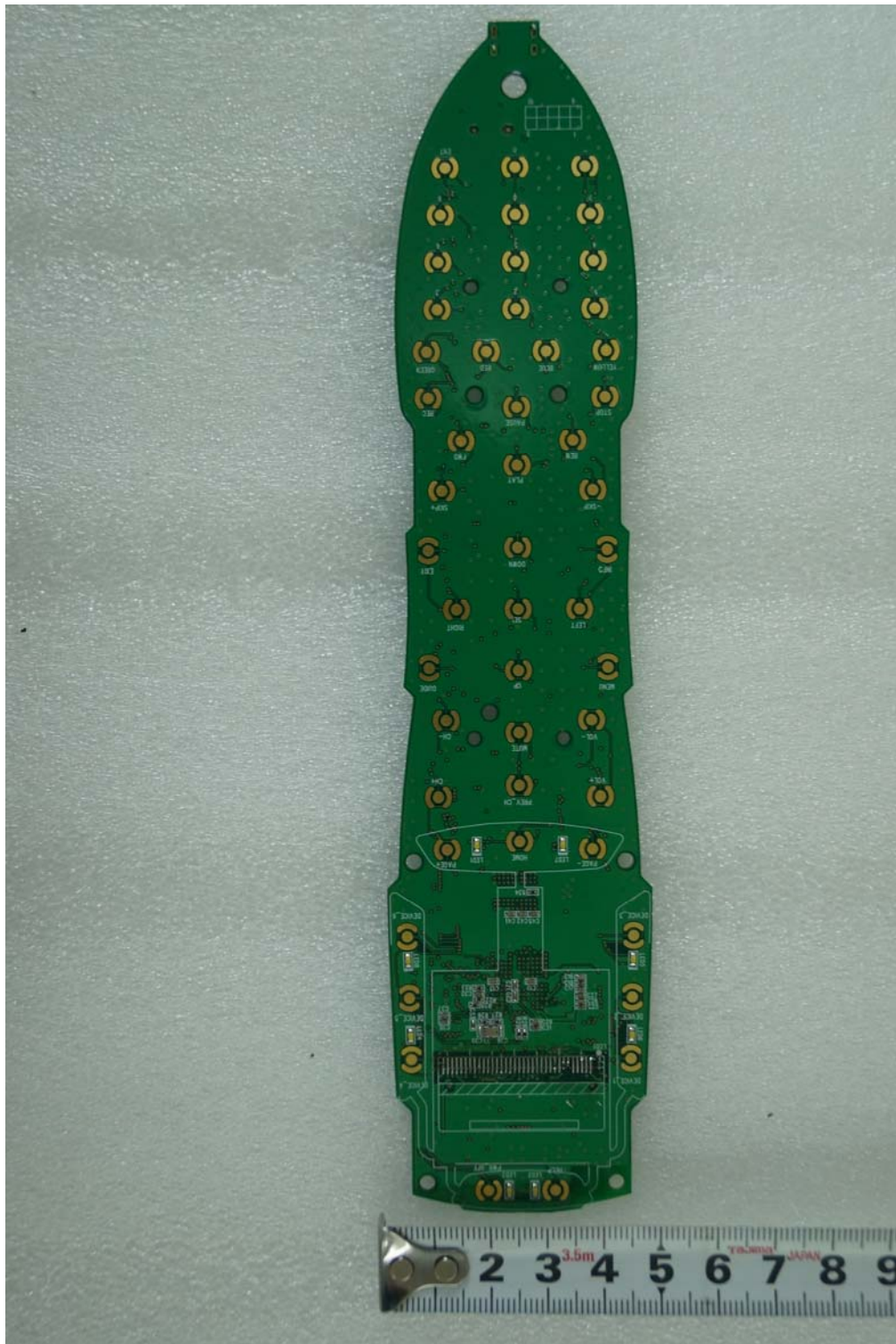
< Main board Bottom view #2 >
