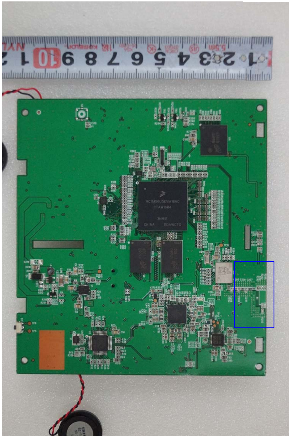
< Original Main board bottom view >
