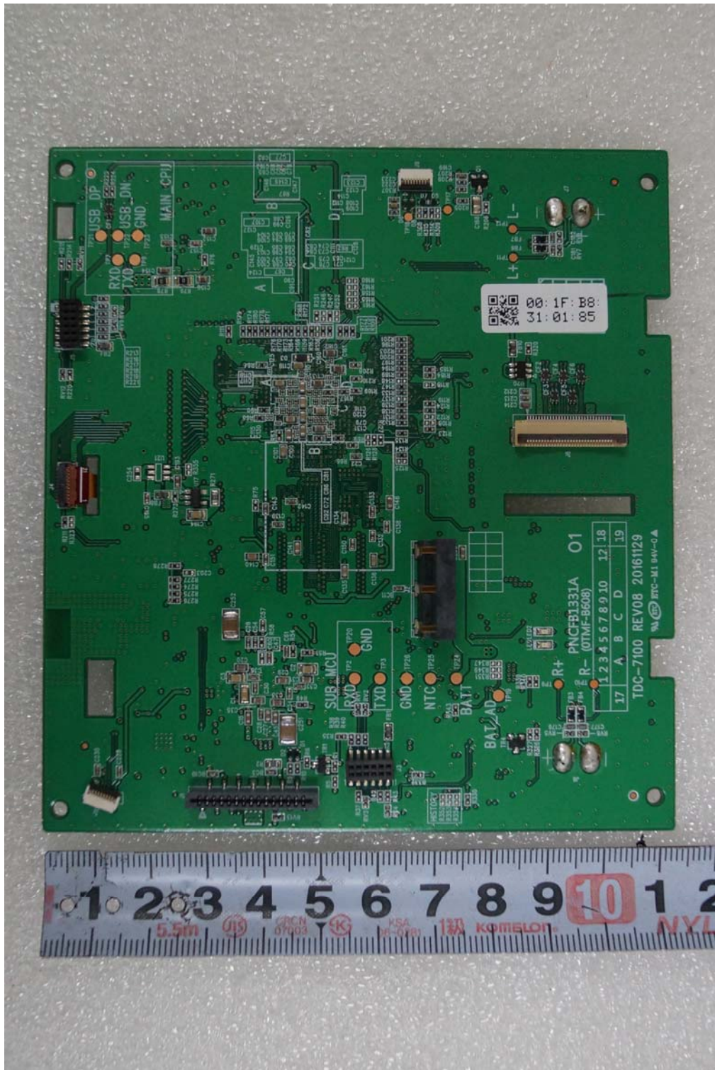
< NEW Main board Top view >
