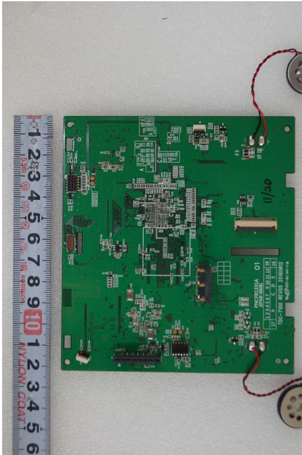
< Original Main board Top view >
