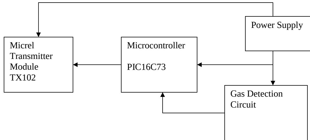
Block Diagram of GSS2001RF Gas Detector Qtronic Manufacture Inc.
