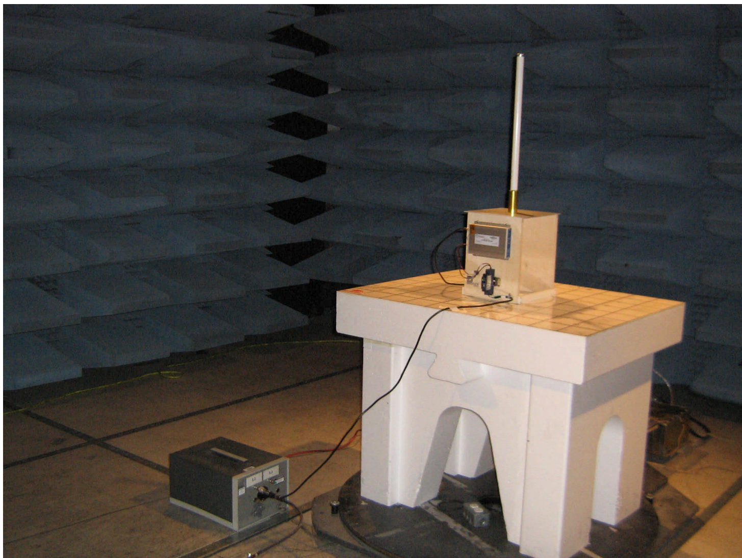
AC Conducted Test Setup
