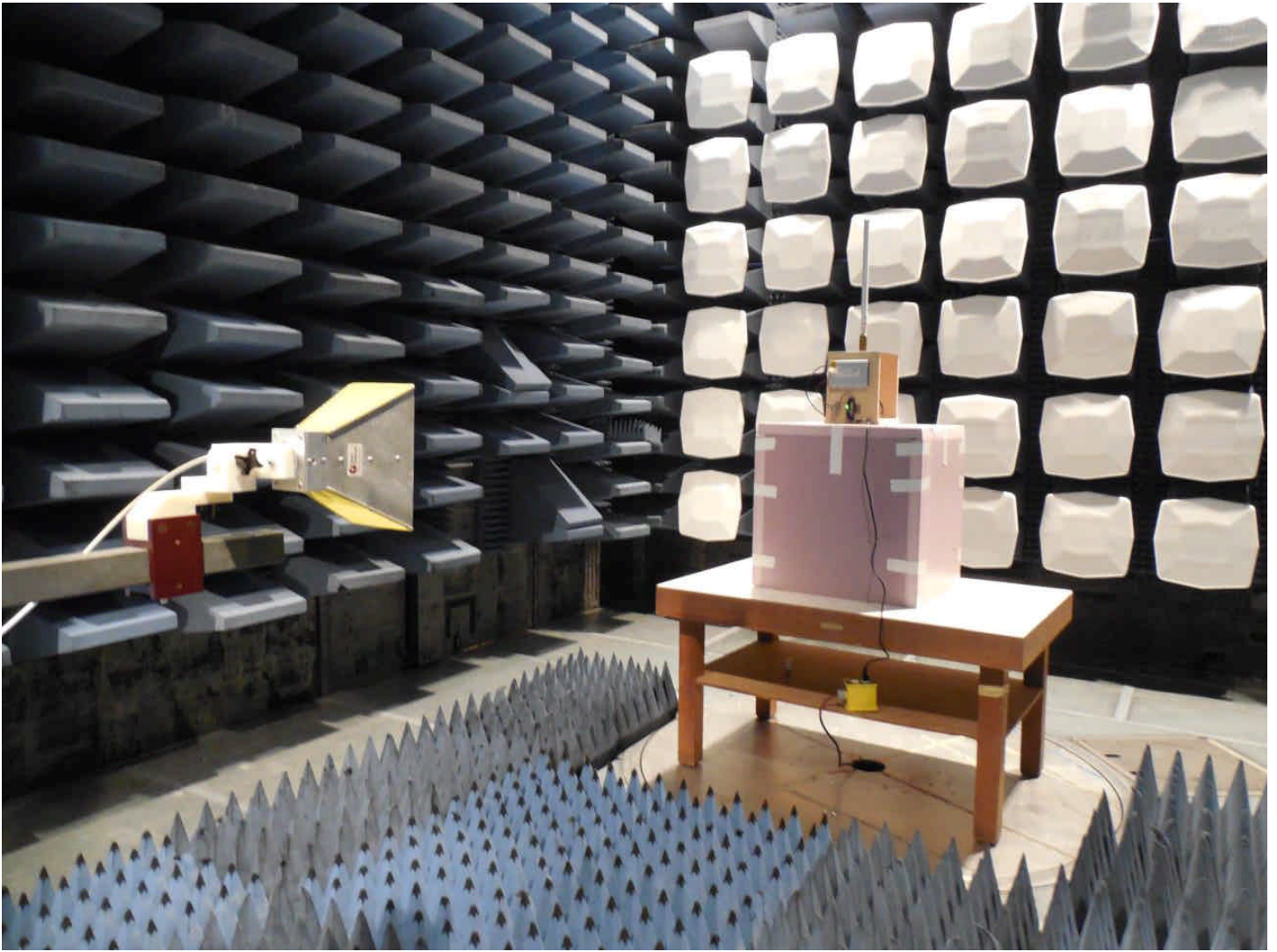
Emissions Test Setup – Intentional/Unintentional Radiated Emissions 1000 - 10000 MHz
