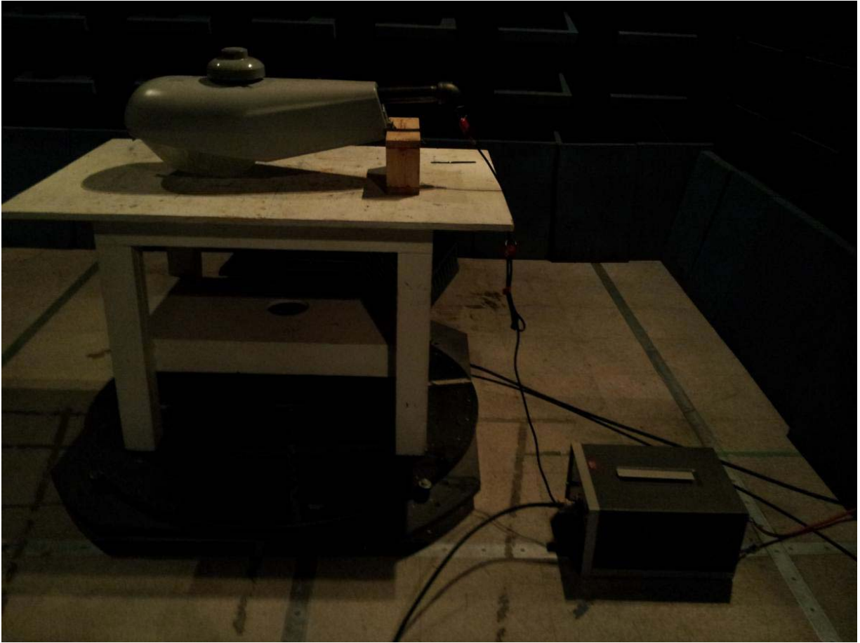
AC Conducted Test Setup
