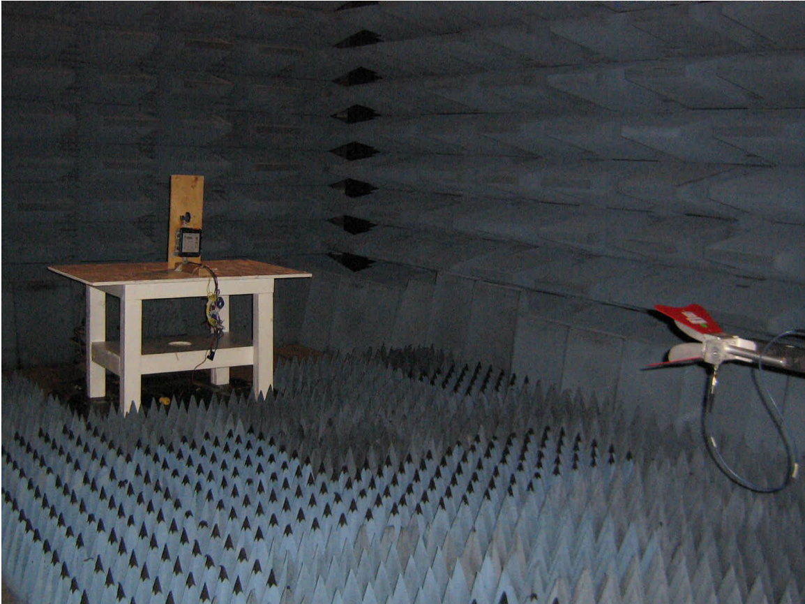
Emissions Test Setup – Intentional/Unintentional Radiated Emissions 1000 - 10000 MHz
