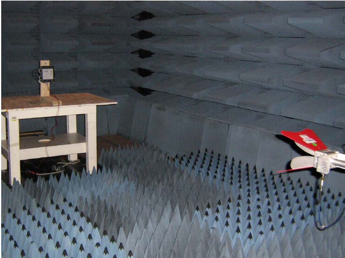
Emissions Test Setup – Intentional Radiated Emissions – Harmonics 1000 - 10000 MHz
