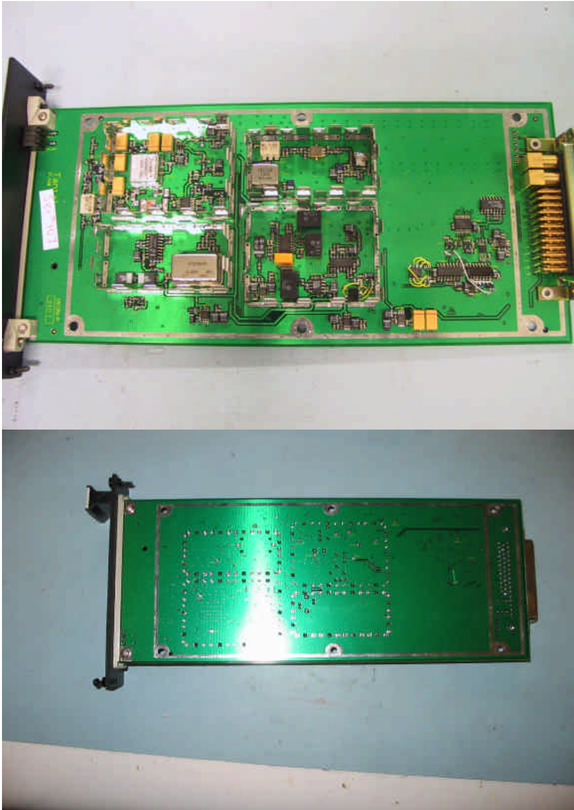
TUNet NC-2200 Network Controller – Receiver Card with shields removed
