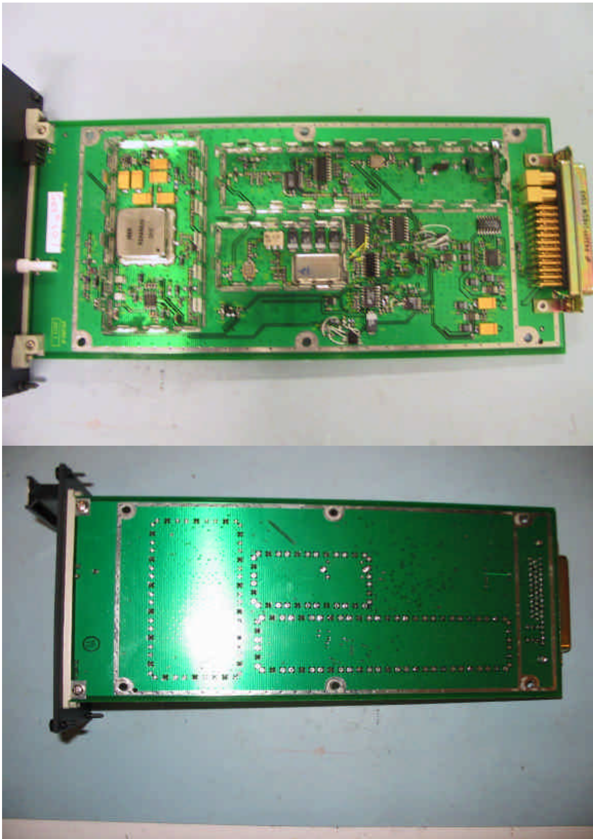
TUNet NC-2200 Network Controller – Transmitter Card with shields removed
