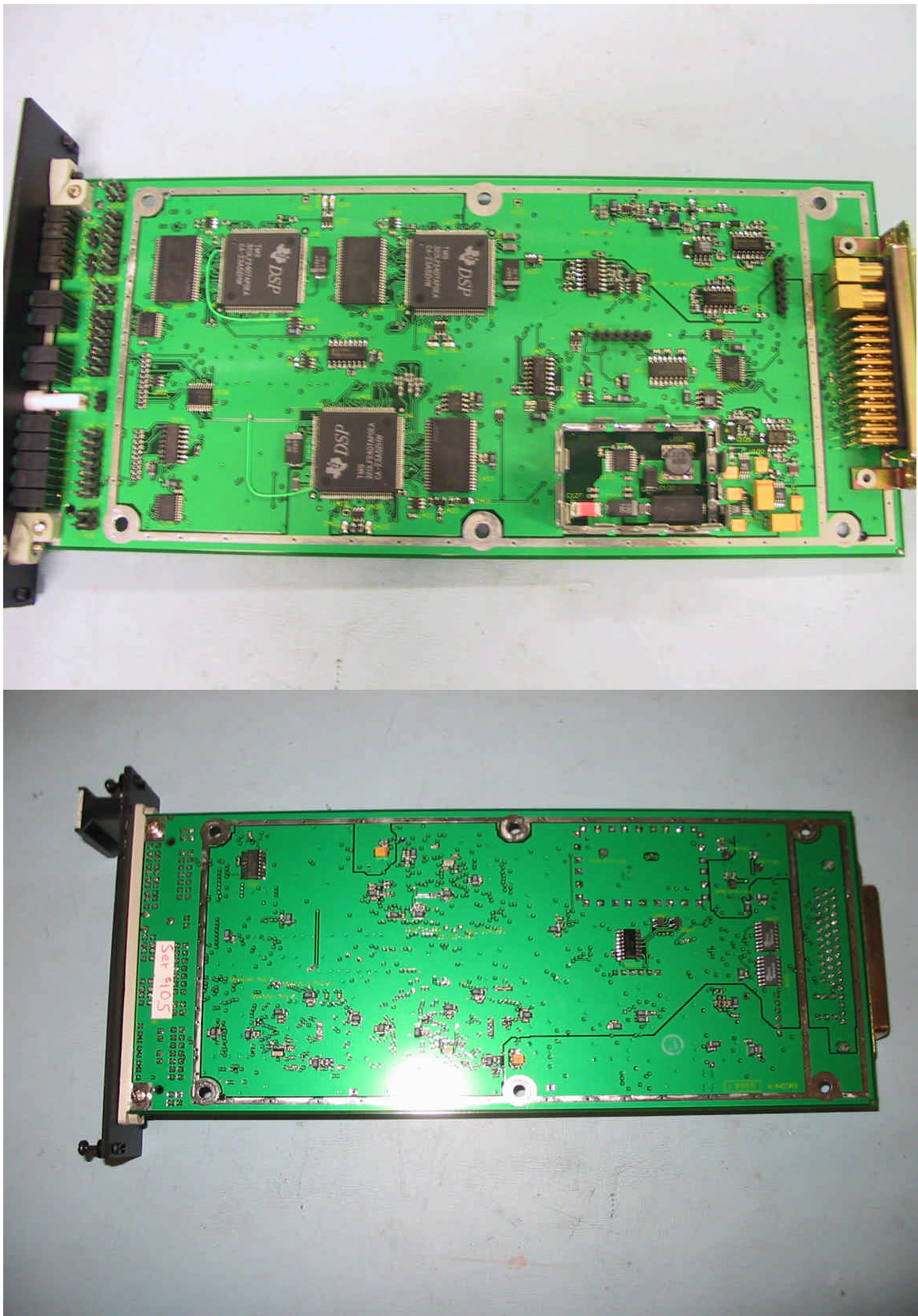
TUNet NC-2202 Network Controller – Controller Card with shields removed
