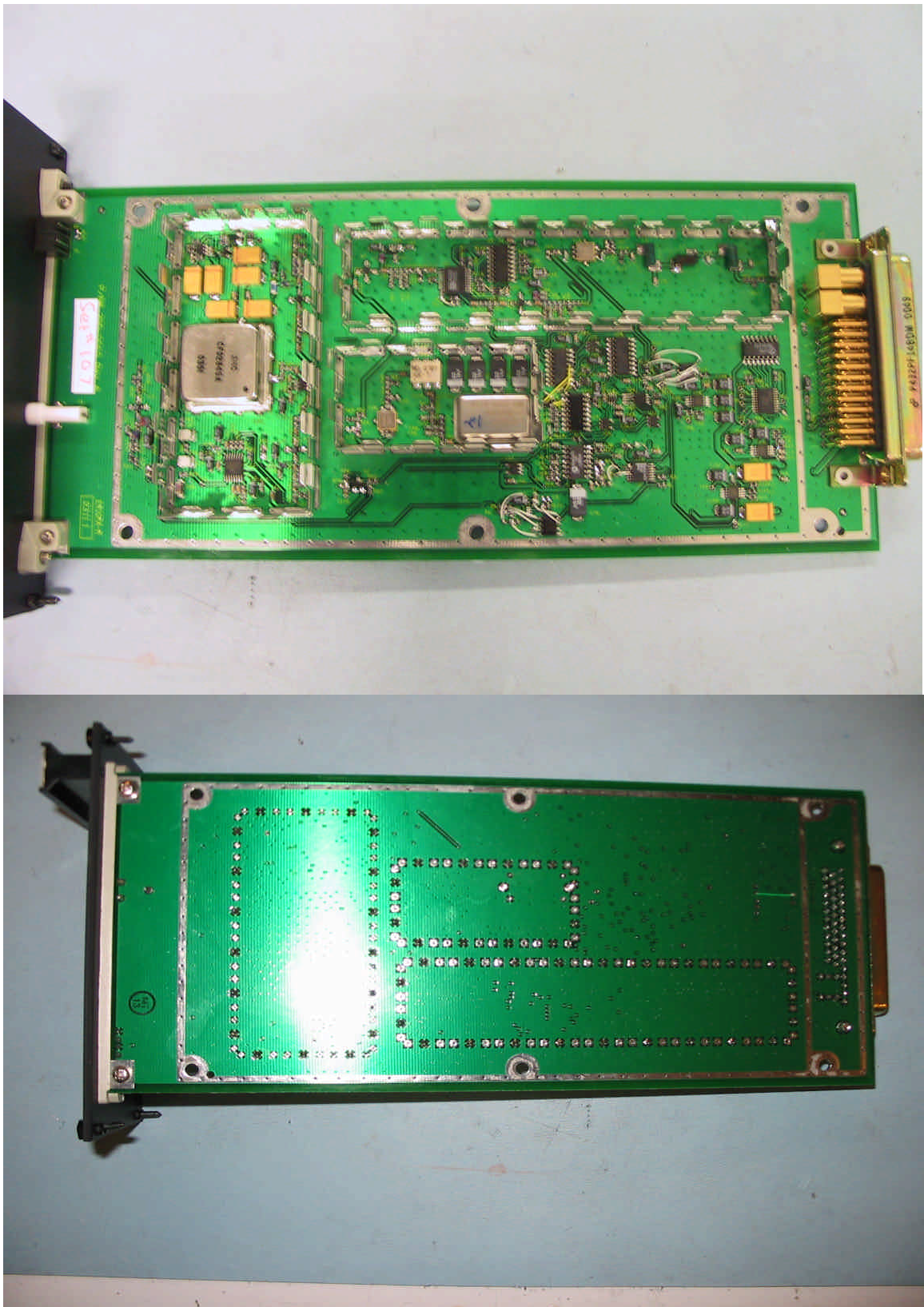
TUNet NC-2202 Network Controller – Transmitter Card with shields removed
