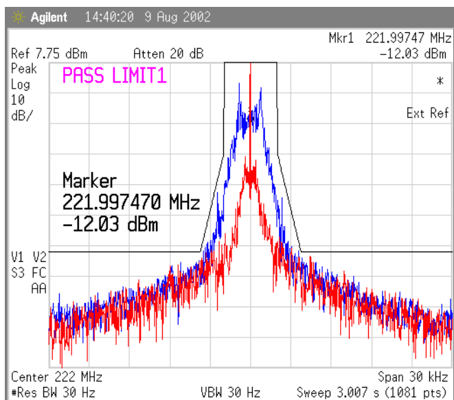
Figure 29 Temp 10 deg Celsius, 1600 bps
