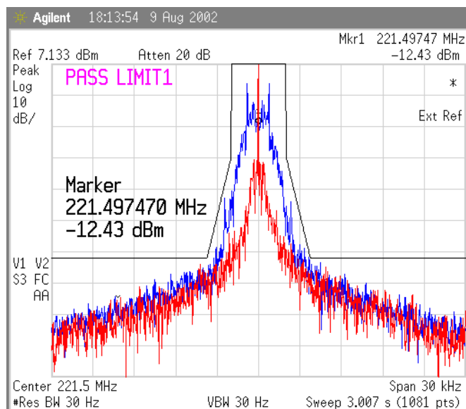
Figure 45 Temp 40 deg Celsius, 1600 bps
