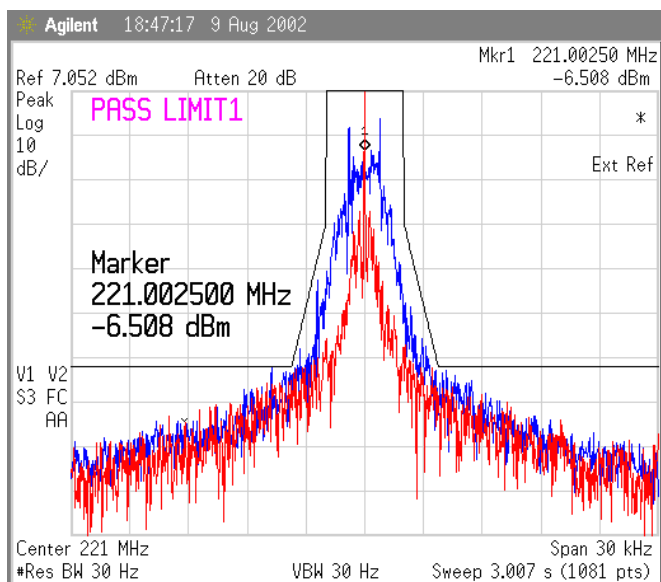
Figure 49 Temp 50 deg Celsius, 1600 bps
