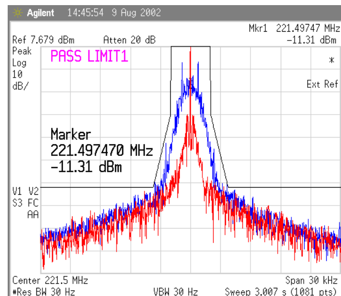
Figure 27 Temp 10 deg Celsius, 1600 bps
