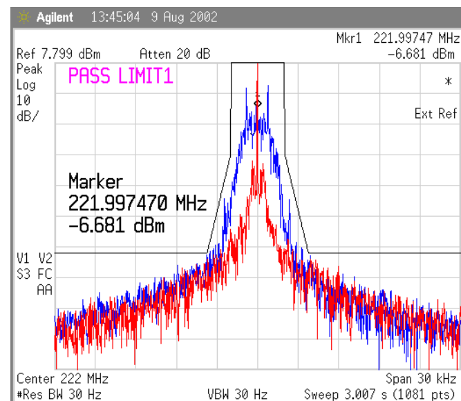
Figure 23 Temp 0 deg Celsius, 1600 bps
