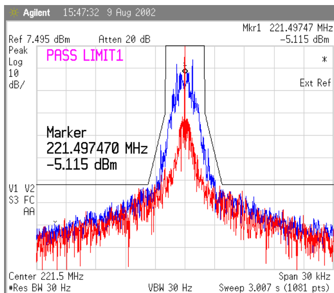
Figure 33 Temp 20 deg Celsius, 1600 bps
