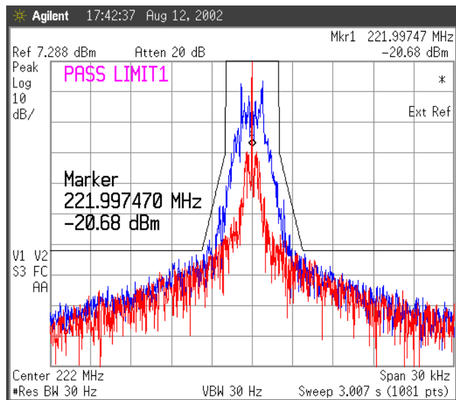
Figure 73 Temp 25 deg Celsius, 1600 bps, 115% Supply Voltage.
