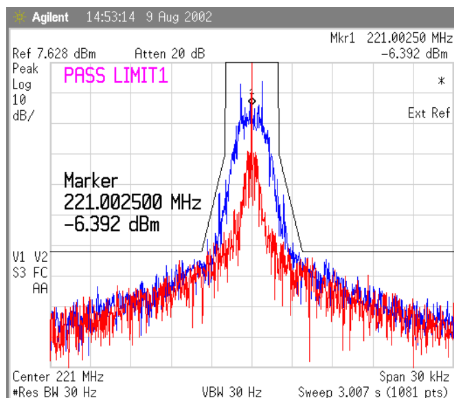
Figure 25 Temp 10 deg Celsius, 1600 bps
