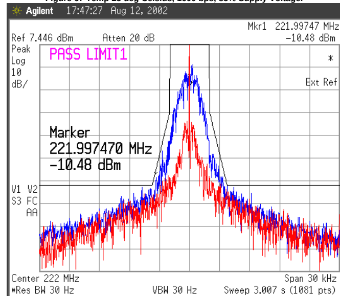
Figure 68 Temp 25 deg Celsius, 1600 bps, 85% Supply Voltage.
