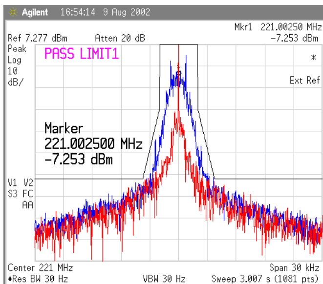
Figure 37 Temp 30 deg Celsius, 1600 bps
