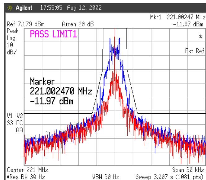
Figure 63 Temp 25 deg Celsius, 1600 bps, 85% Supply Voltage
