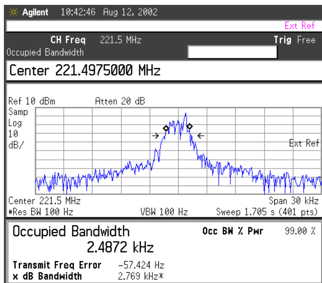
Figure 61 Temp 25 deg Celsius, 1600 bps
