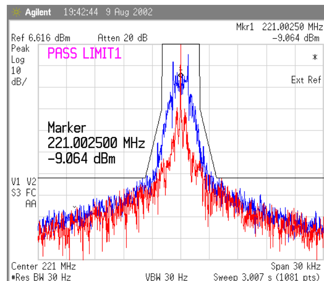
Figure 55 Temp 60 deg Celsius, 1600 bps
