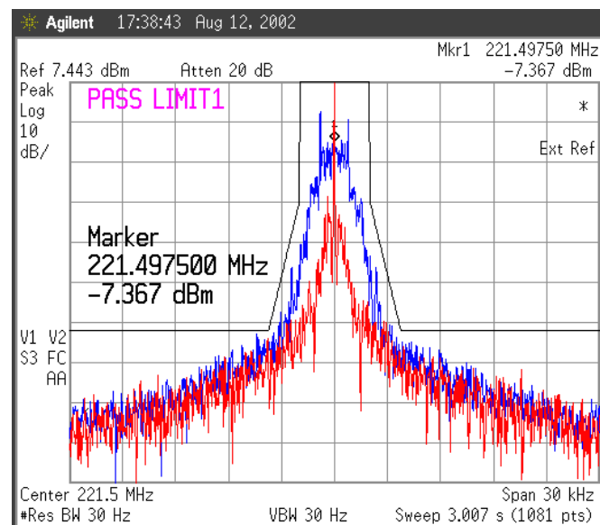
Figure 71 Temp 25 deg Celsius, 1600 bps, 115% Supply Voltage.
