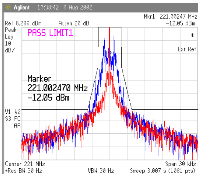
Figure 1 Temp -30 deg Celsius, 1600 bps
