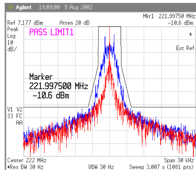
Figure 47 Temp 40 deg Celsius, 1600 bps
