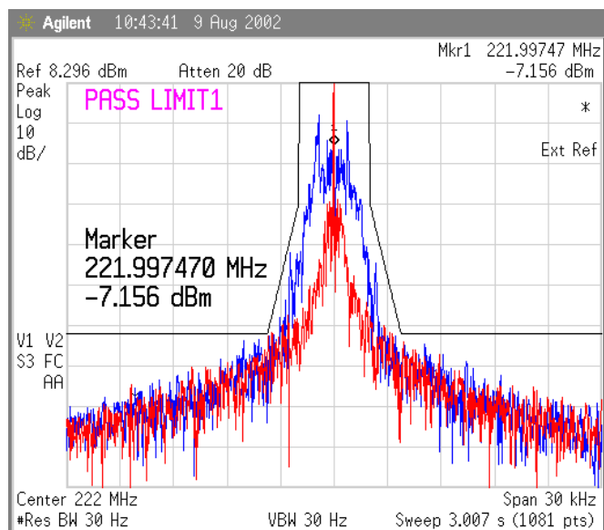
Figure 5 Temp -30 deg Celsius, 1600 bps
