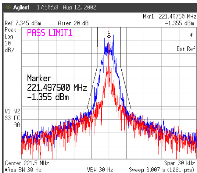
Figure 65 Temp 25 deg Celsius, 1600 bps, 85% Supply Voltage.
