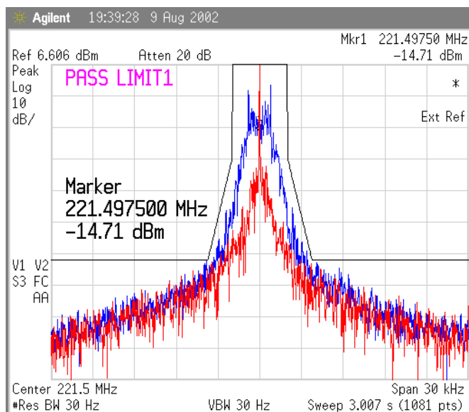
Figure 57 Temp 60 deg Celsius, 1600 bps
