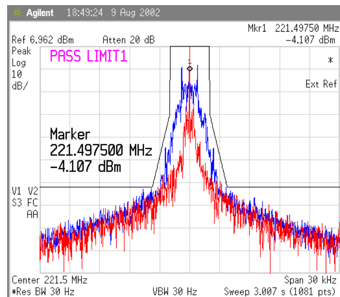
Figure 51 Temp 50 deg Celsius, 1600 bps
