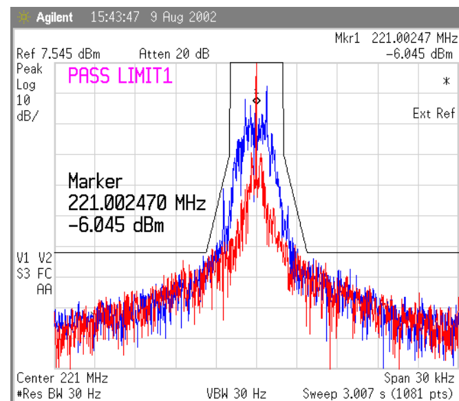
Figure 7 Temp -20 deg Celsius, 1600 bps
