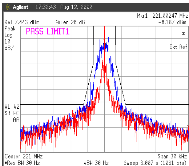
Figure 69 Temp 25 deg Celsius, 1600 bps, 115% Supply Voltage.
