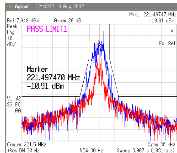
Figure 15 Temp -10 deg Celsius, 1600 bps
