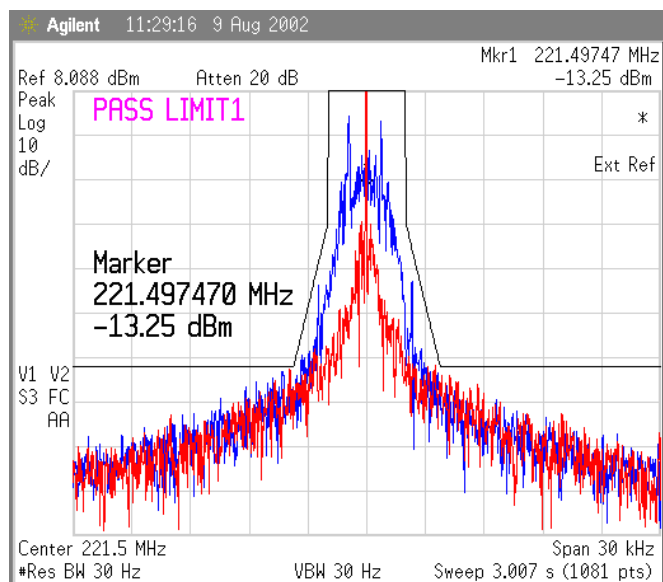
Figure 9 Temp -20 deg Celsius, 1600 bps
