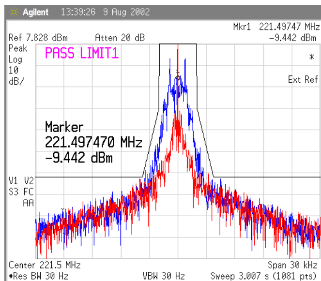
Figure 21 Temp 0 deg Celsius, 1600 bps
