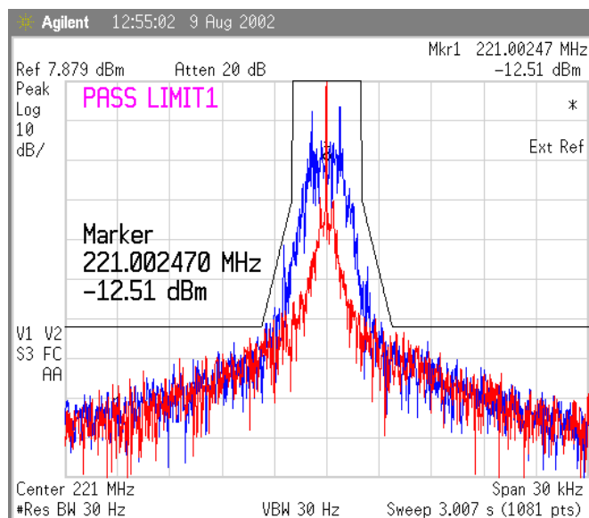
Figure 13 Temp -10 deg Celsius, 1600 bps
