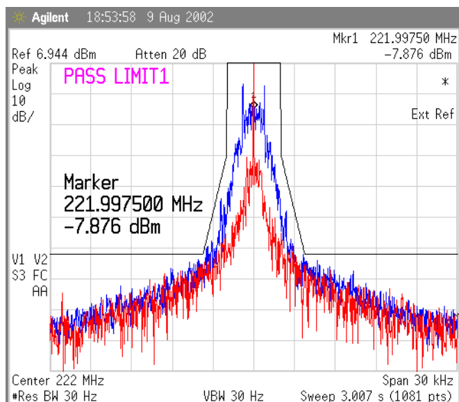
Figure 53 Temp 50 deg Celsius, 1600 bps
