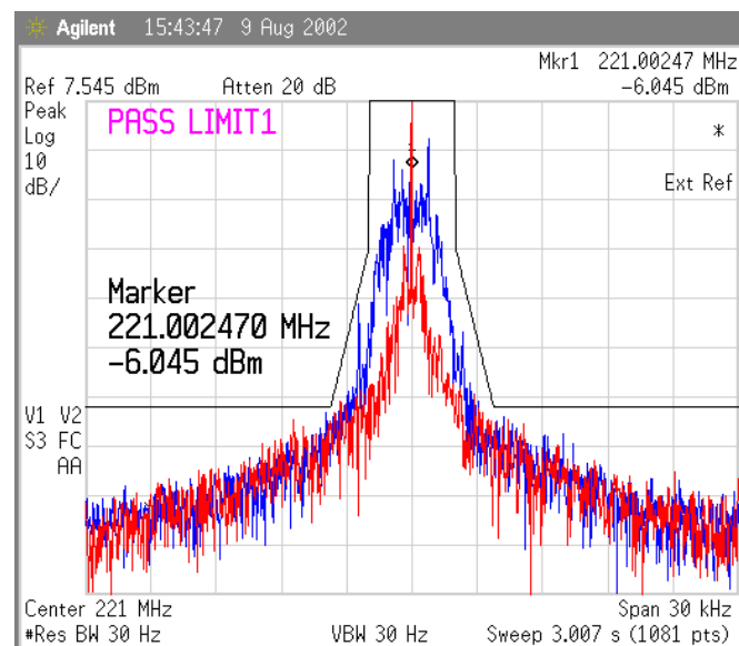
Figure 31 Temp 20 deg Celsius, 1600 bps
