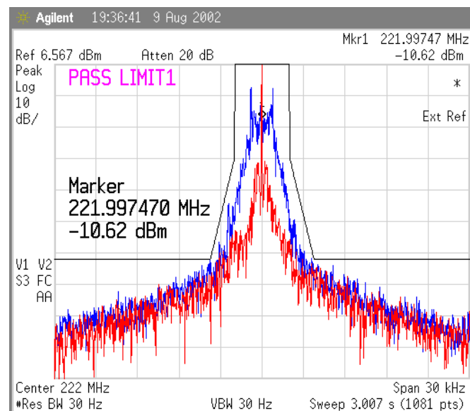
Figure 59 Temp 60 deg Celsius, 1600 bps
