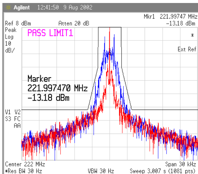
Figure 17 Temp -10 deg Celsius, 1600 bps
