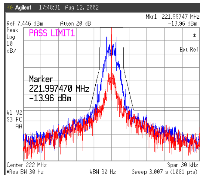
Figure 67 Temp 25 deg Celsius, 1600 bps, 85% Supply Voltage.
