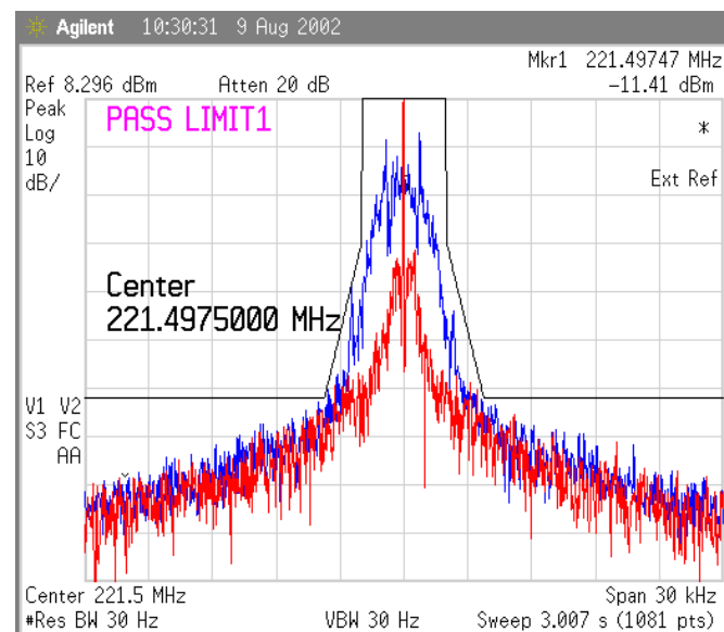
Figure 3 Temp -30 deg Celsius, 1600 bps
