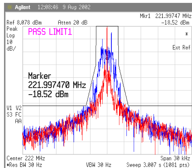
Figure 11 Temp -20 deg Celsius, 1600 bps
