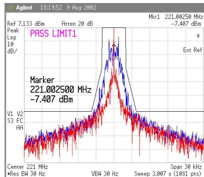
Figure 43 Temp 40 deg Celsius, 1600 bps
