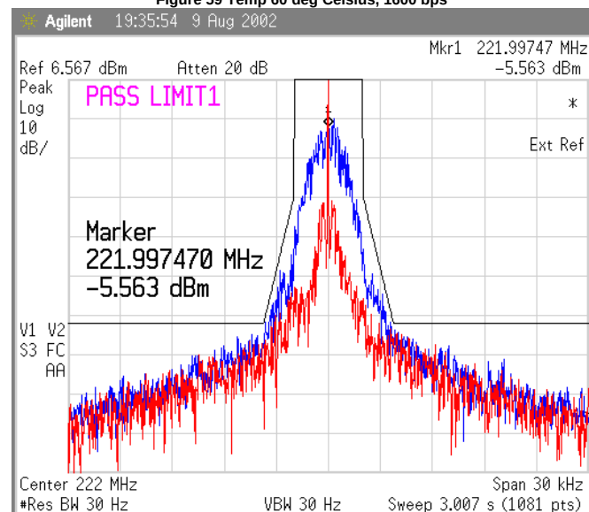
Figure 60 Temp 60 deg Celsius, 3200 bps
