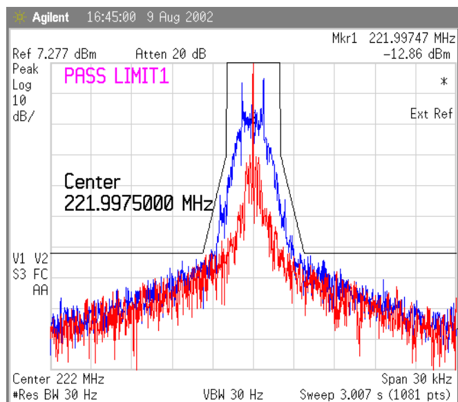
Figure 41 Temp 30 deg Celsius, 1600 bps
