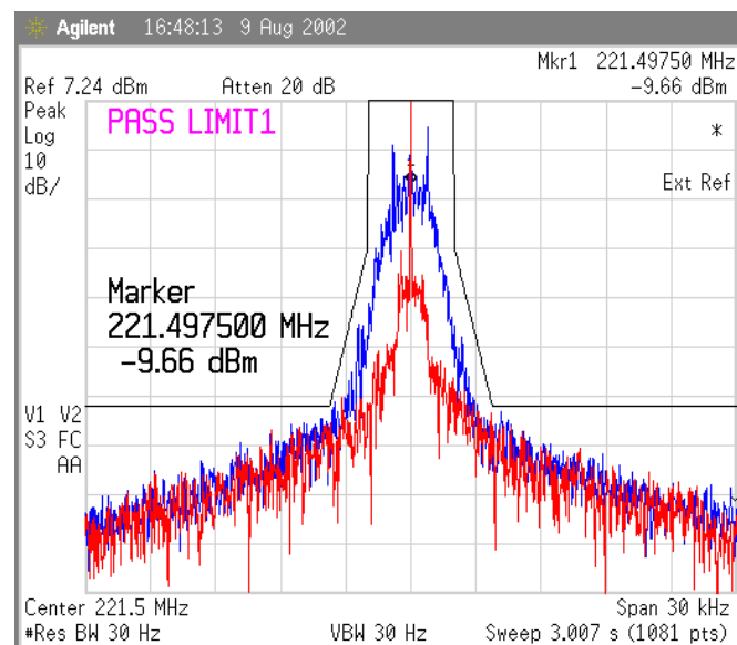
Figure 39 Temp 30 deg Celsius, 1600 bps
