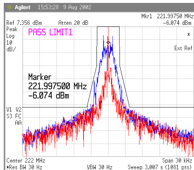
Figure 35 Temp 20 deg Celsius, 1600 bps
