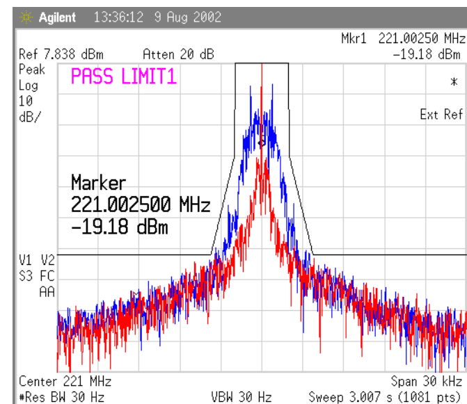
Figure 19 Temp 0 deg Celsius, 1600 bps
