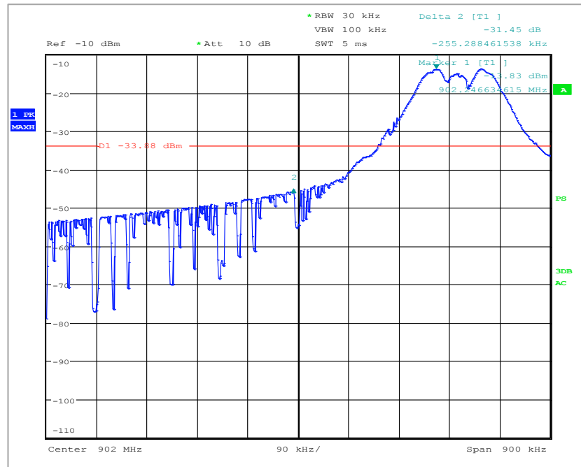
Plot 14: Band Edge Plot (Low Channel ~902.2MHz)
