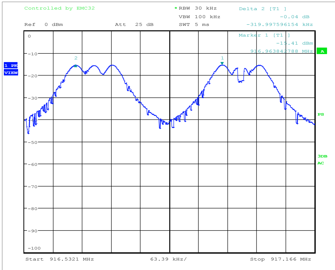
Plot 18: Channel Separation → 320 kHz
