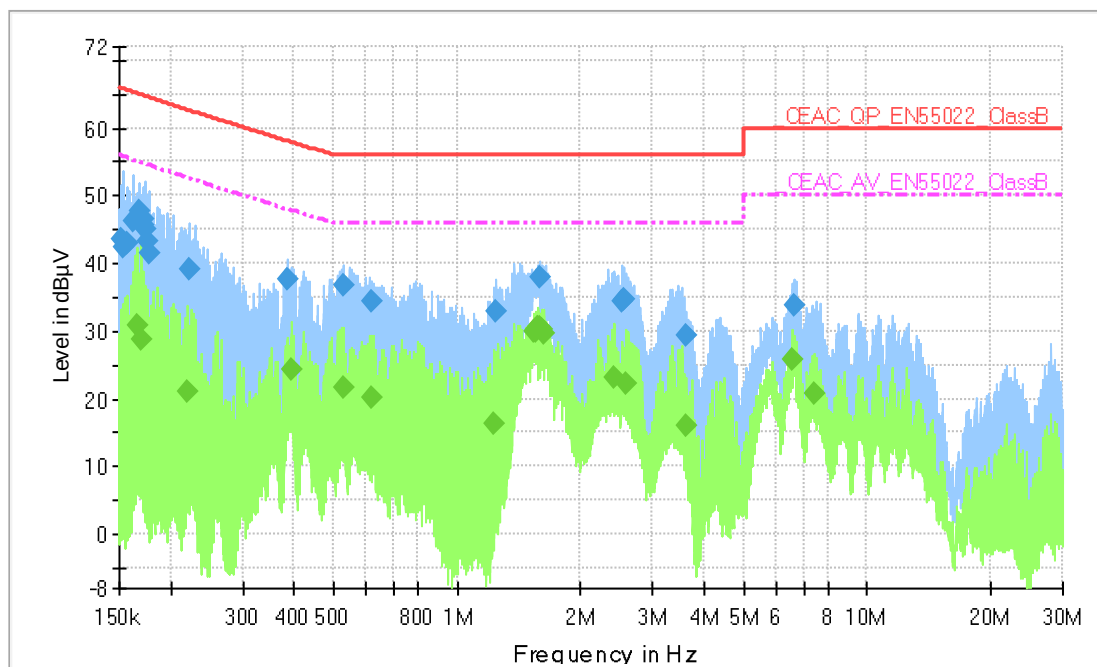
Figure 5: 240V AC Conducted Emissions - Line 1 and Line 2
