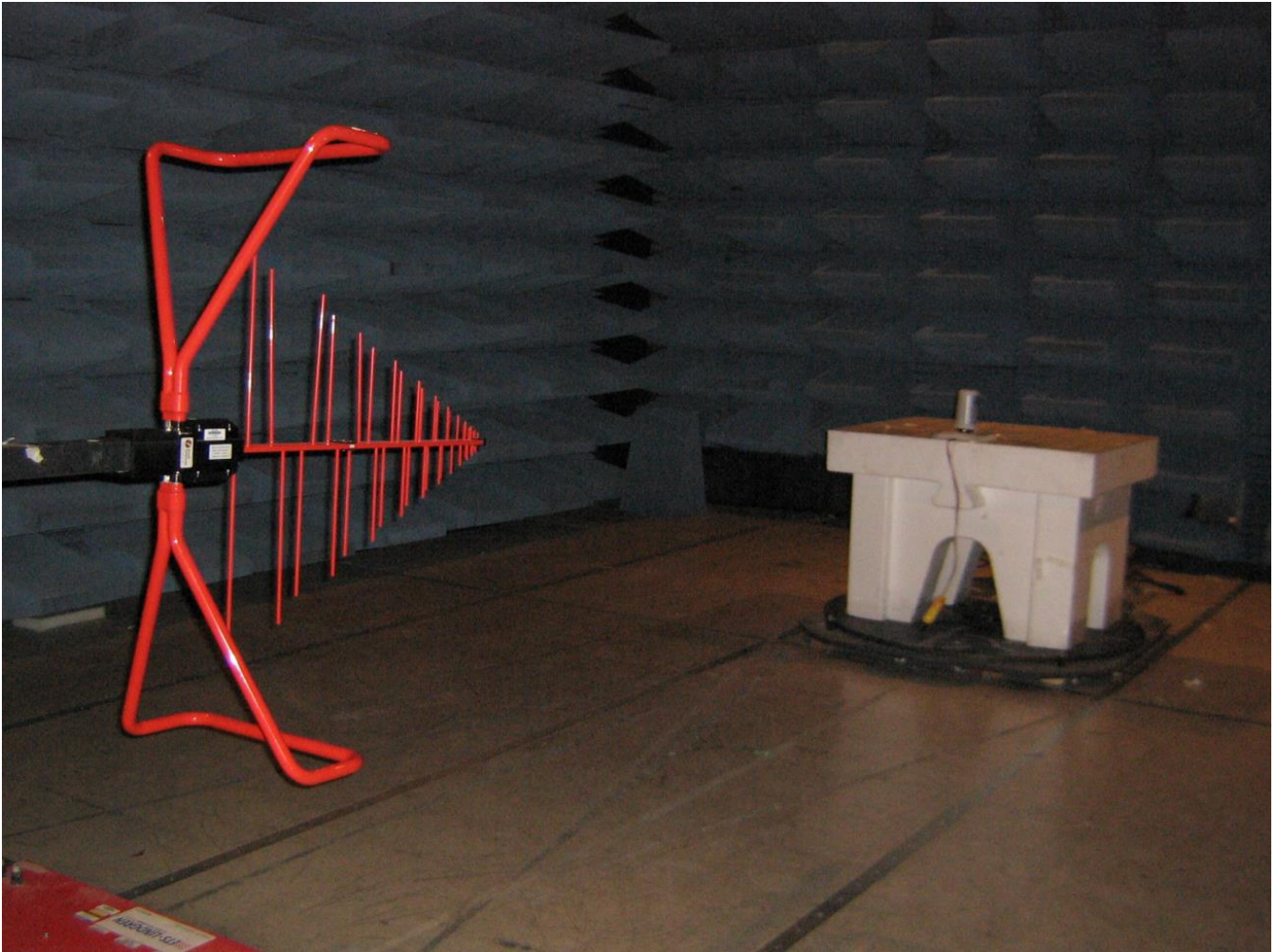
Figure 52: Emissions Test Setup – Intentional / Unintentional Radiated Emissions
