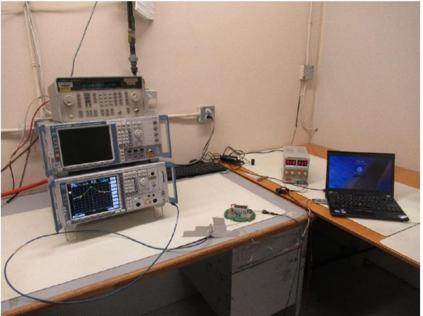
FCC Part 15.247 Conducted RF measurements
