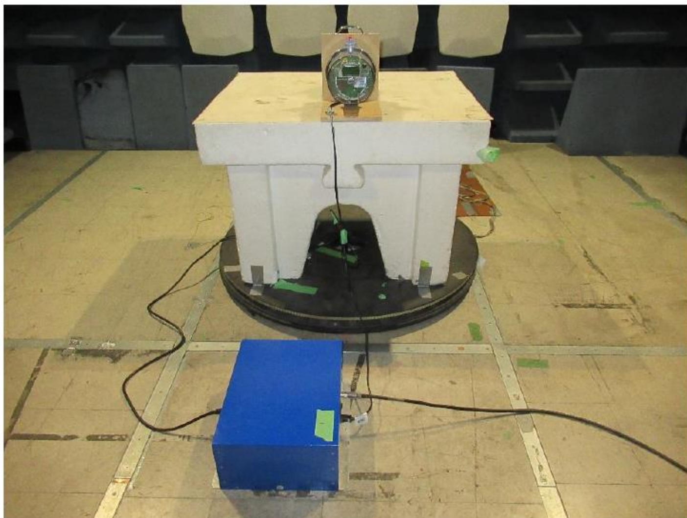
AC conducted Emissions Test Setup
