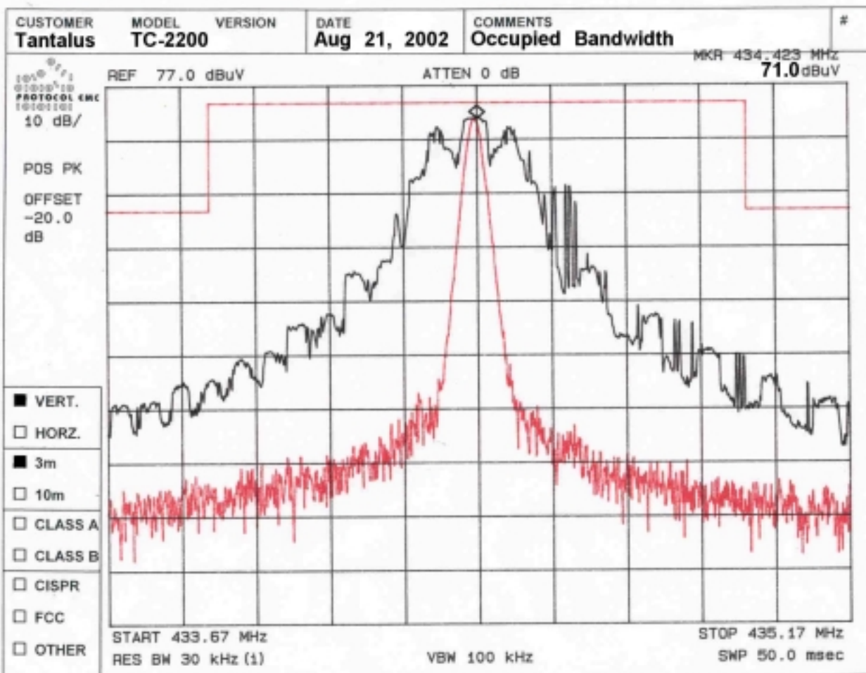
Occupied Bandwidth Plot
