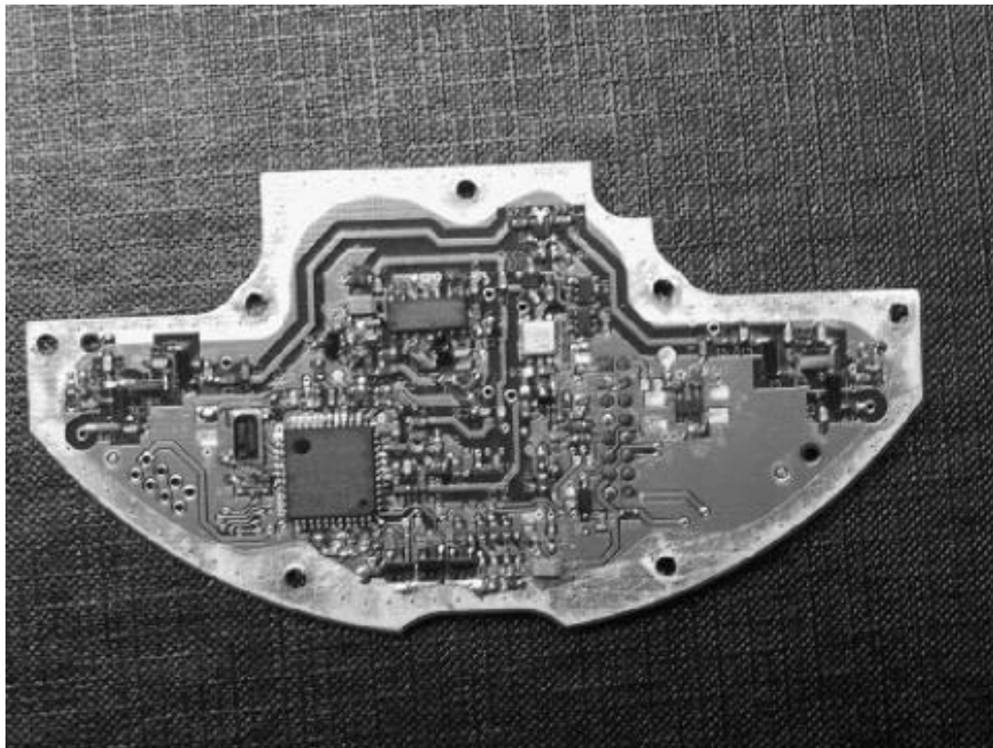
TRANSCEIVER MODULE TOP SIDE
