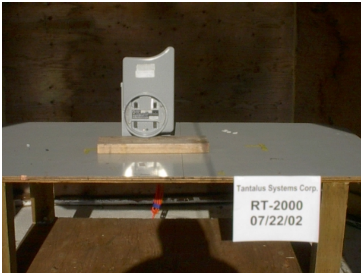
Emissions Test Setup Front View
