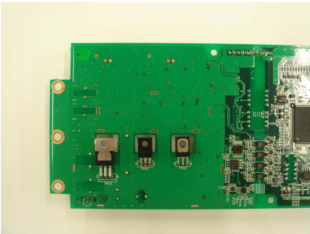
Enlarged wireless part (Rear)
