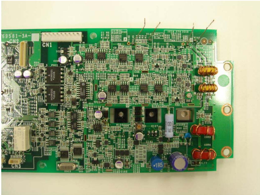
Enlarged wireless part (Front)
