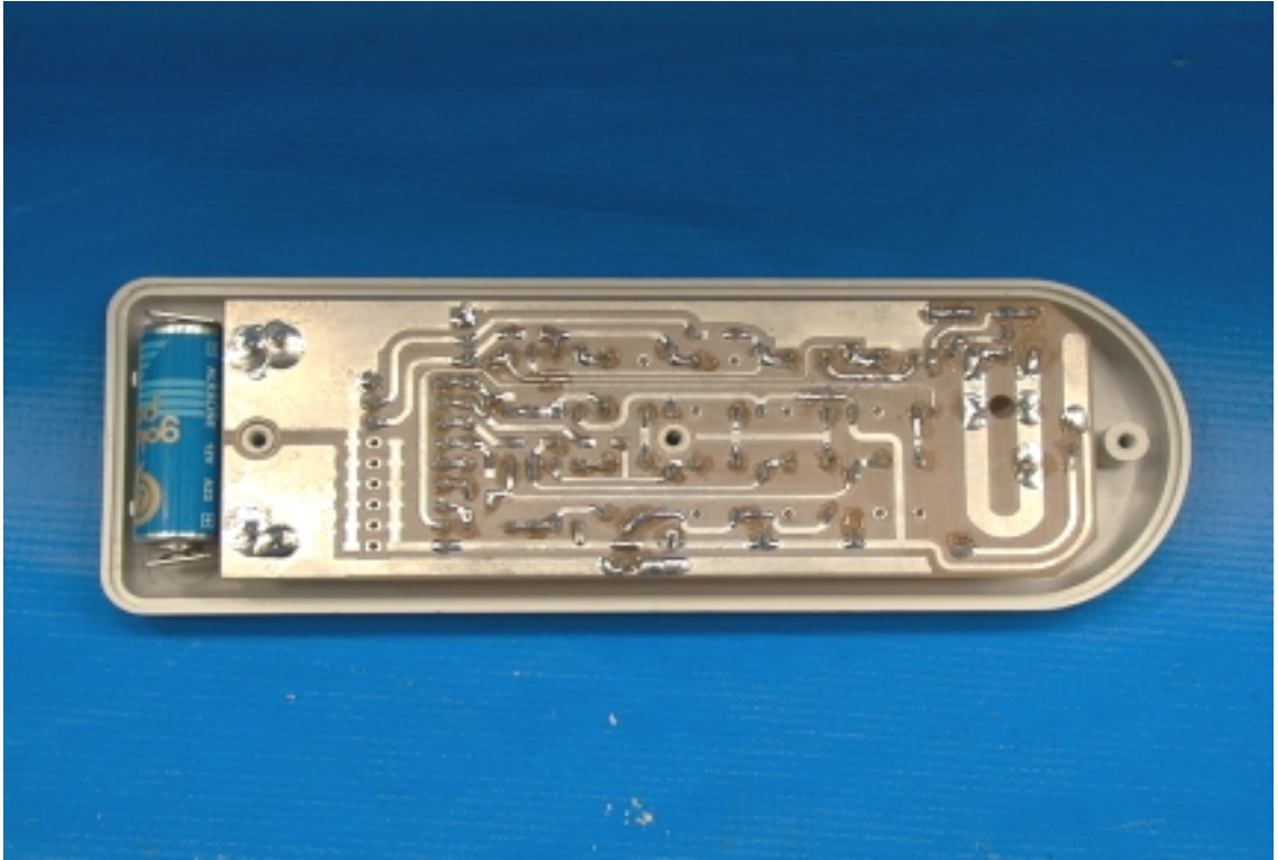
Figure 6.3 EUT Inside View
