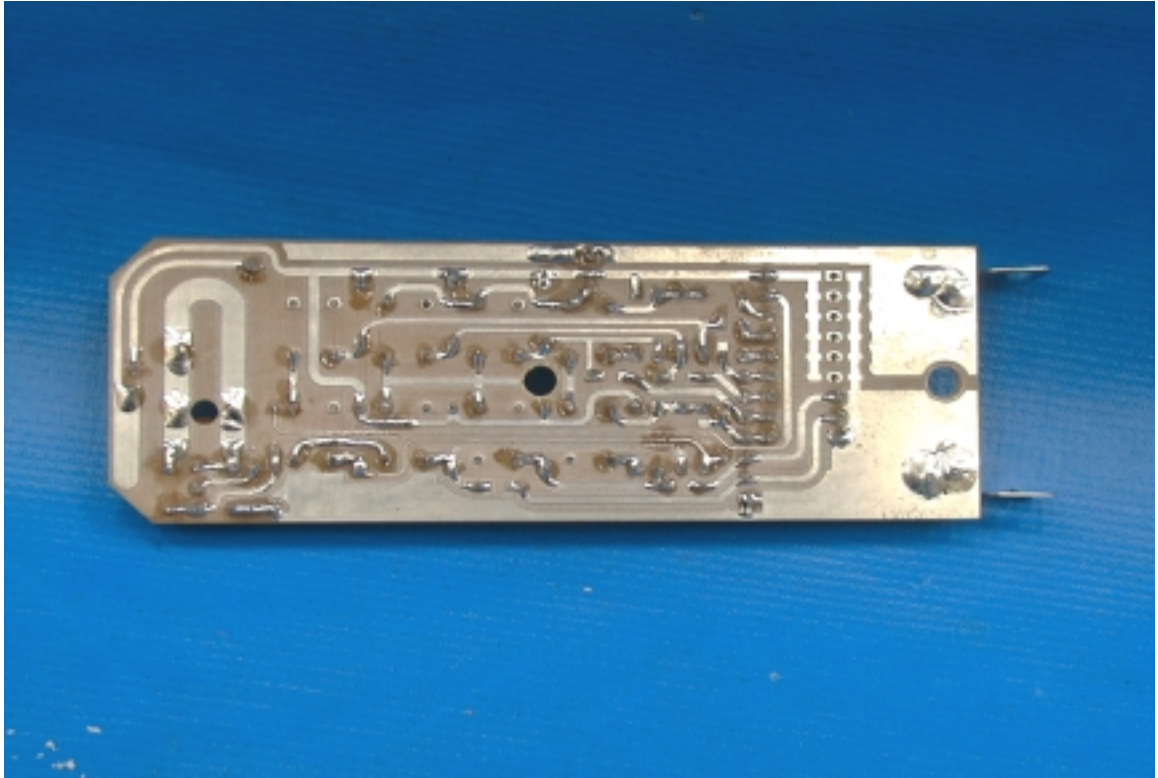
Figure 6.5 EUT Soldering Side View
