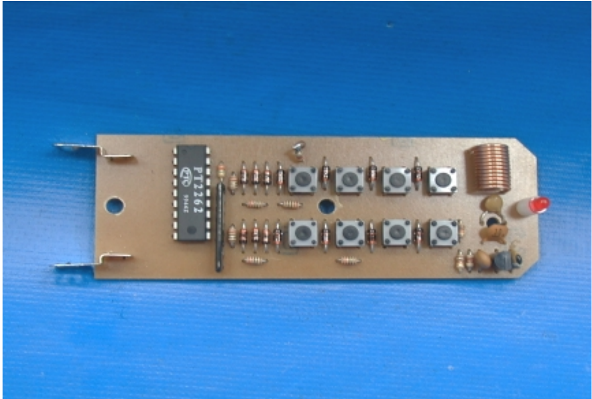
Figure 6.4 EUT Component Side View
