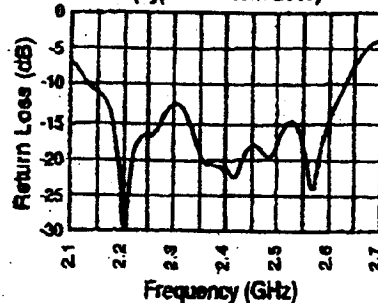
(Typical Return Loss) APG24
