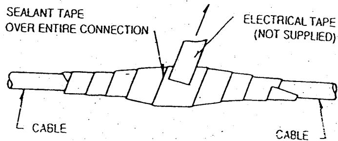
FIG. 2 STRETCH TO ELONGATE ELECTRICAL TAPE WHILE WRAPPING OVER SEALANT TAPE
