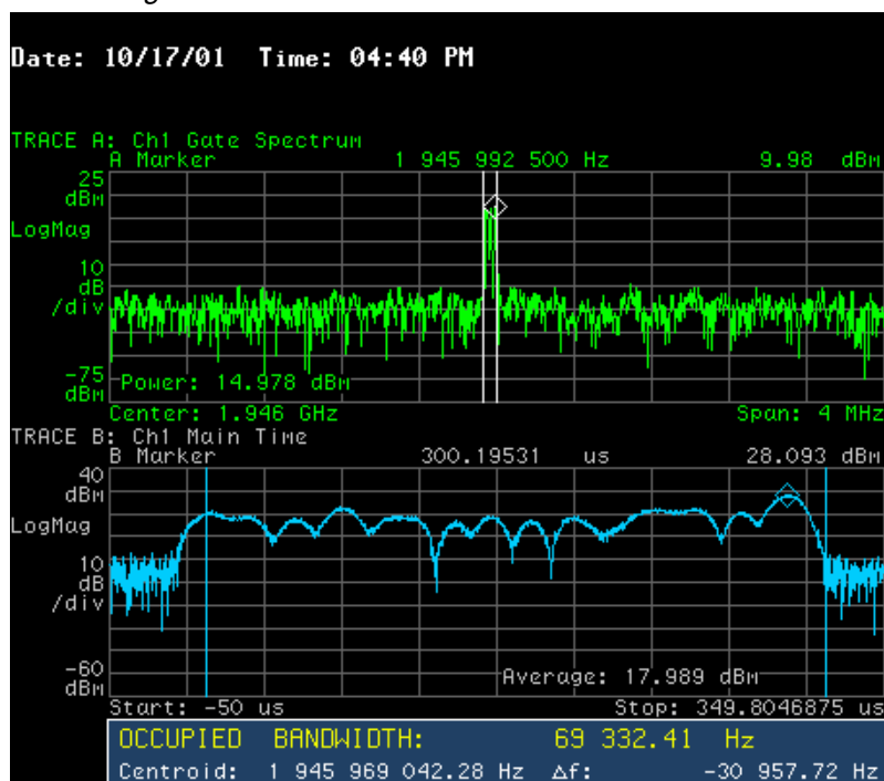
Figure 11.23 NAC Channel Power vs. Frequency, 99.0% Occupied BW, and Time-Domain Average Power.
