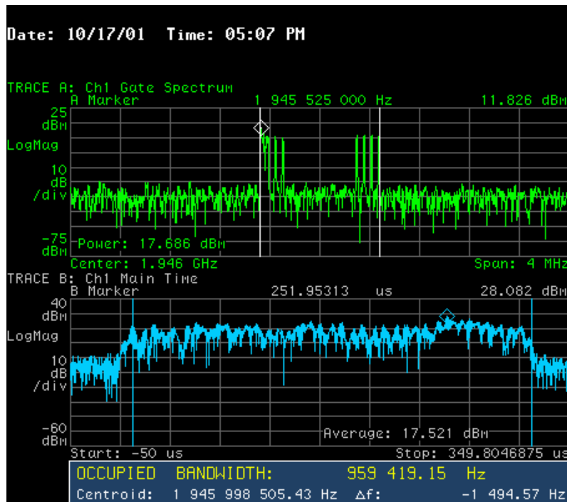
Figure 11.27 Simulcast Remote Synchronization Pilots Power vs. Frequency, 99.0% Occupied Bandwidth, and Time-Domain Average Burst Power.
