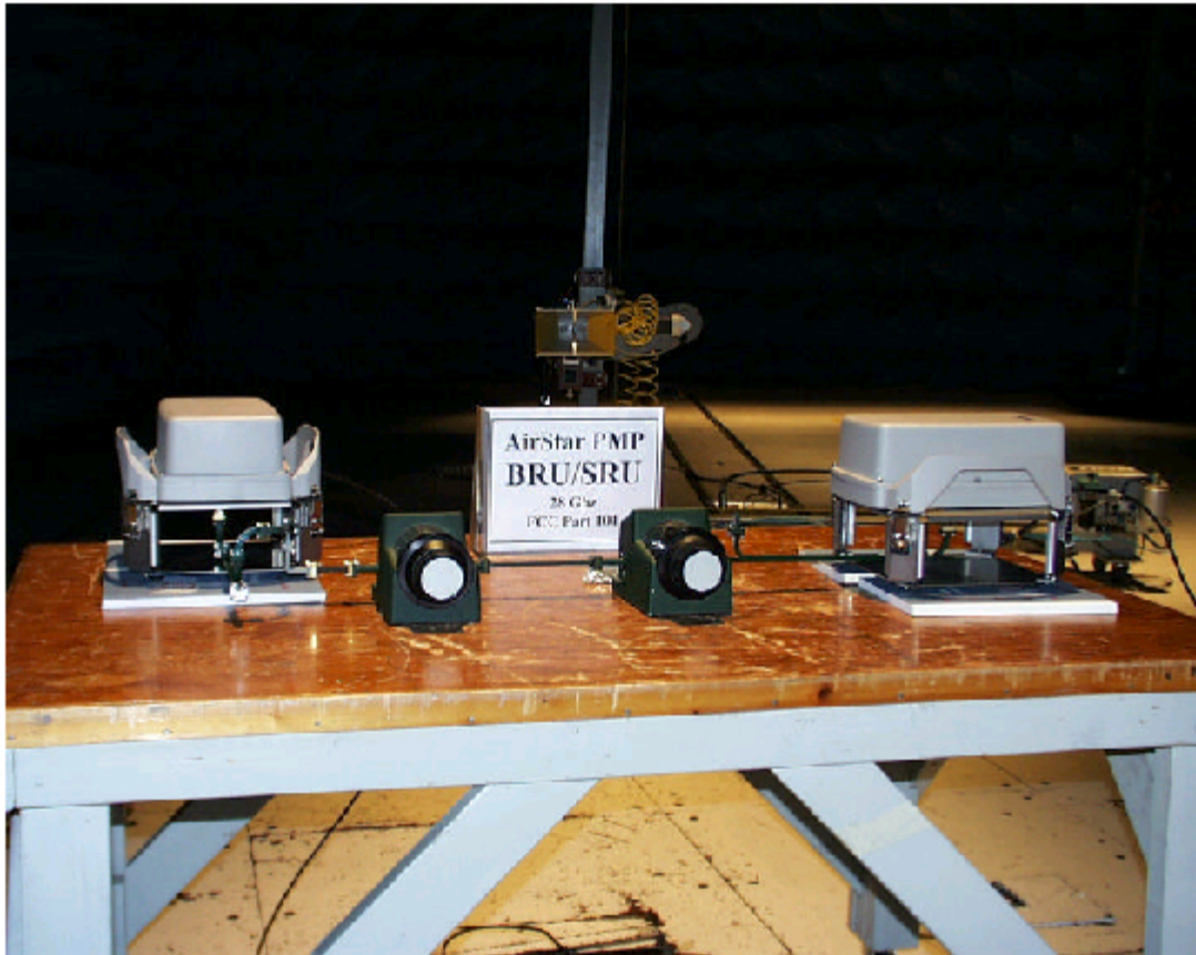
Photograph of Test Setup: Radiated Emissions 30 MHz - 1000 MHz
