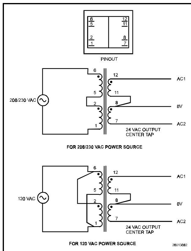
Figure 2-2 - Pinout for the 175VA (640-0048) Transformer
