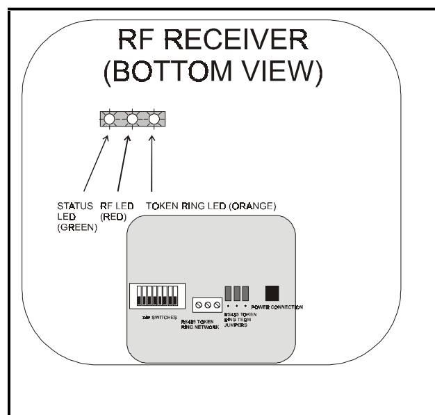
Figure 7-1 - RF Receiver LED Locations
