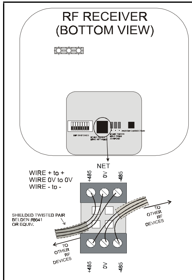
Figure 3-1 - Connecting the RF Receiver to the RS485 Network
