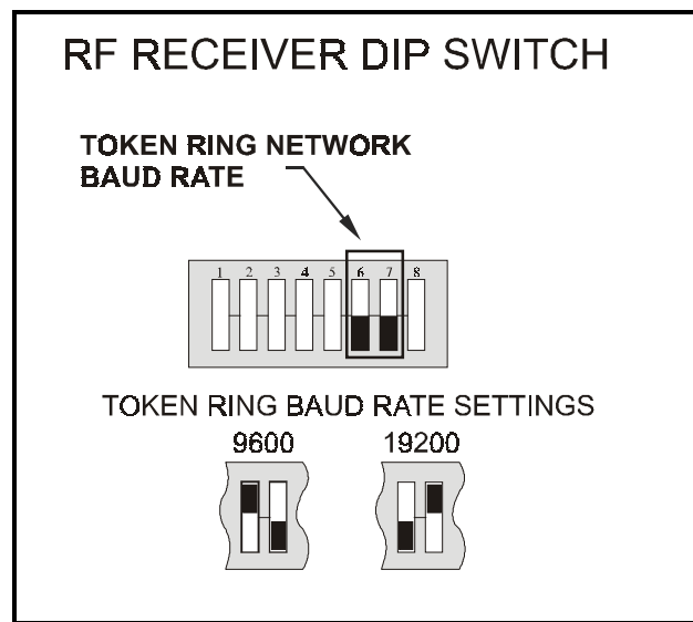
Figure 3-4 - Dip Switch Setting for RF Receiver Baud Rate
