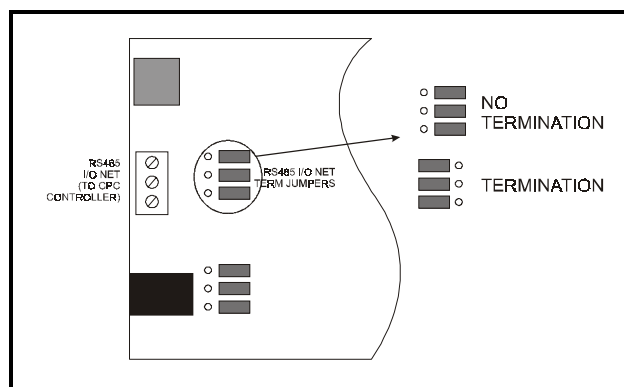
Figure 2-6 - RF Gateway RS485 I/O Network Termination
