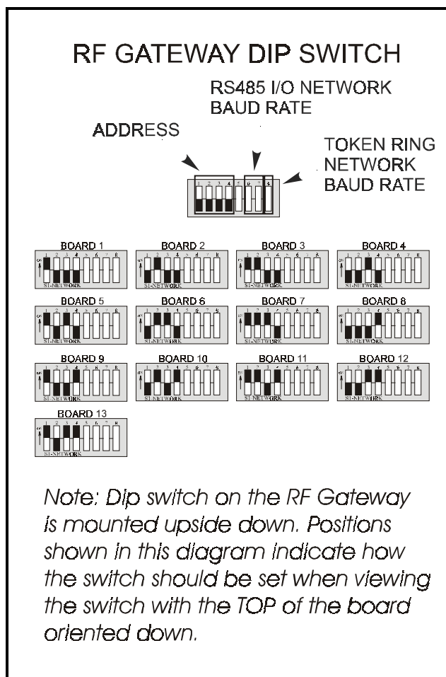
Figure 2-4 - Dip Switch Setting for Numbering RF Gateway
