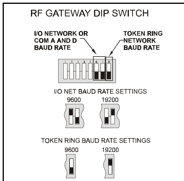
Figure 2-5 - Dip Switch Setting for Numbering RF Gateway
