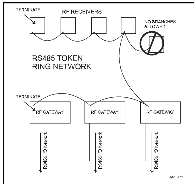
Figure 2-7 - Daisy Chain Configuration - Token Ring Network
