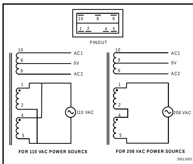
Figure 2-1 - Pinout for the 56VA (640-0043) and 100VA (640-0045) Transformers
