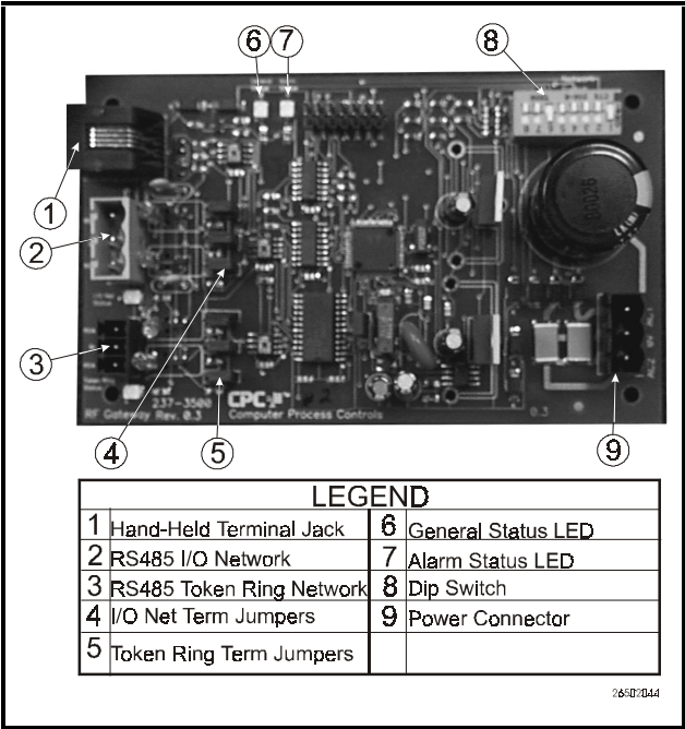
Figure 1-6 - RF Gateway Board
