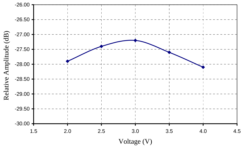
Figure 6.5. Relative emission at 433.92 MHz vs. supply voltage (pulsed emission).
