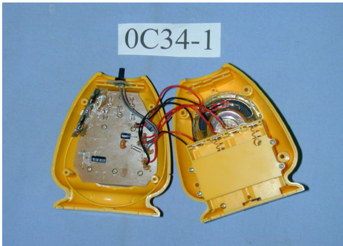
Receiver case inside whole view
