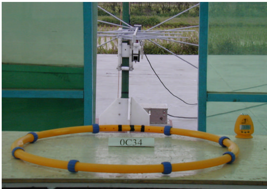
Open site test back view
