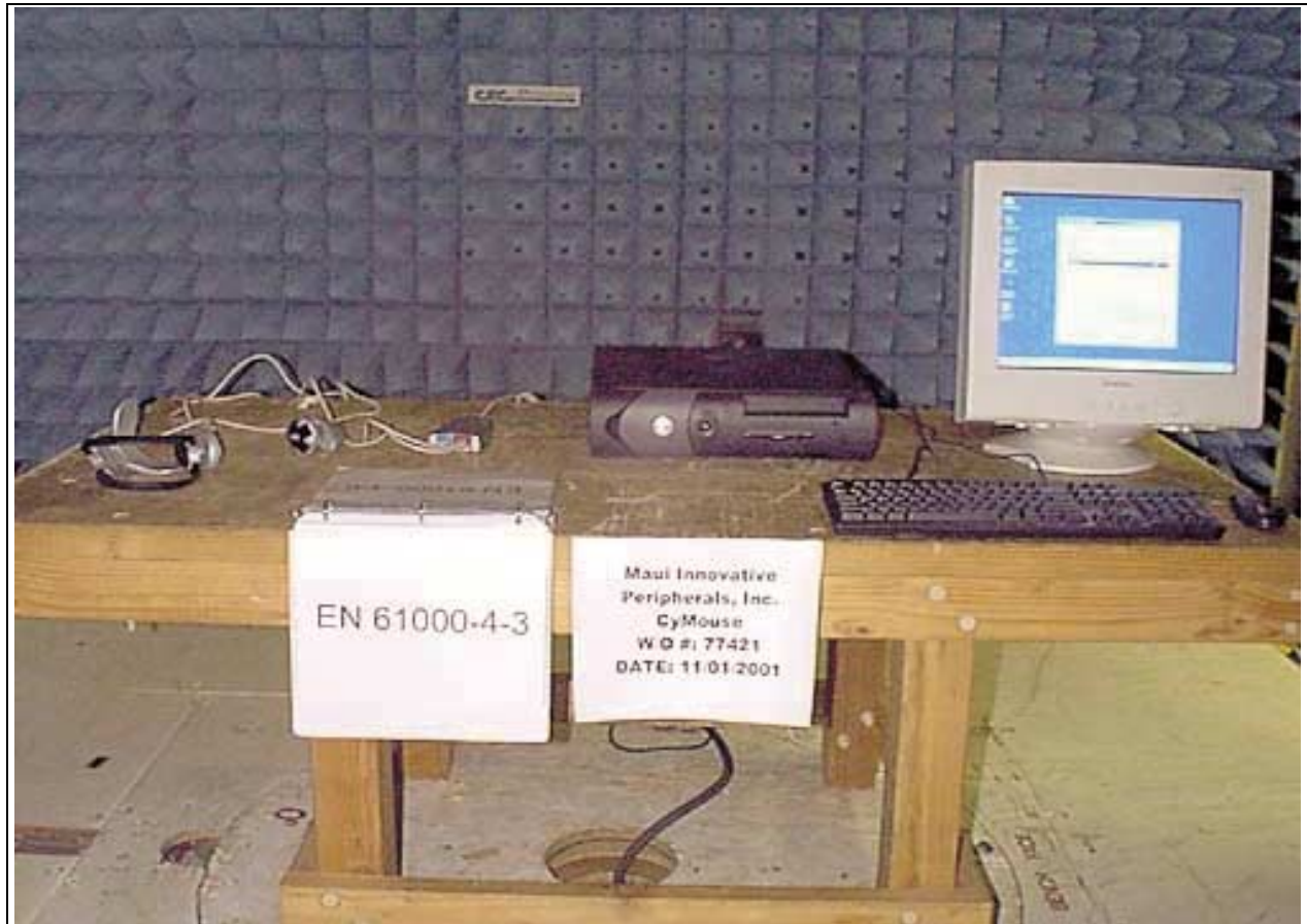
Radiated Immunity - Front View
