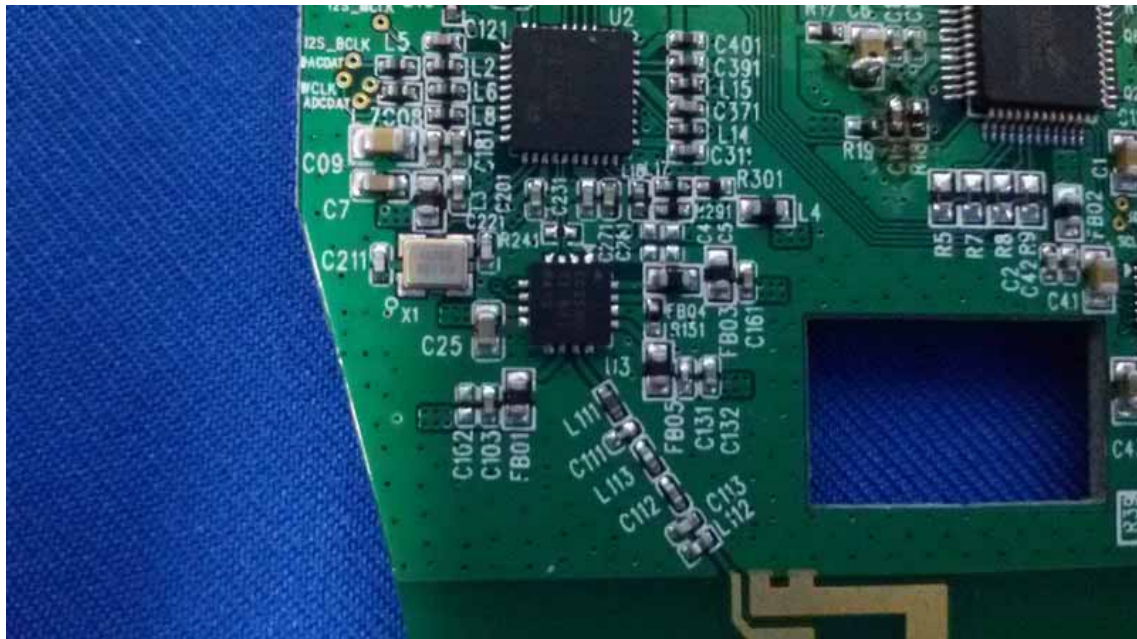
Figure 22 Inside of the EUT
