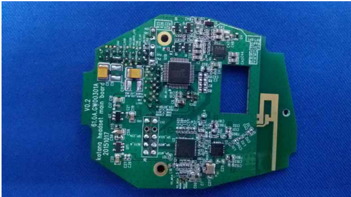
Figure 19 Inside of the EUT
